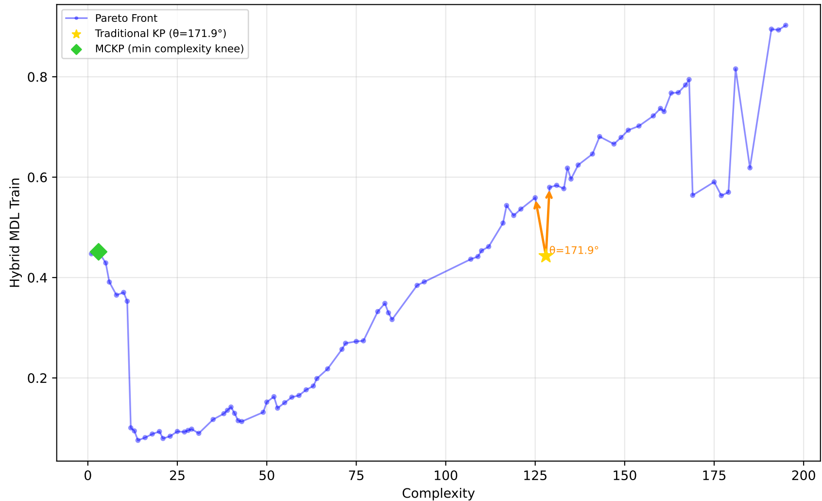
557_analcatdata_apnea1 - Run 3 - MVP - Hybrid MDL Train \lambda_1=0.00, \lambda_2=0.00, \lambda_3=0.00 | Difficulty: 0.85 | Method: hmr
