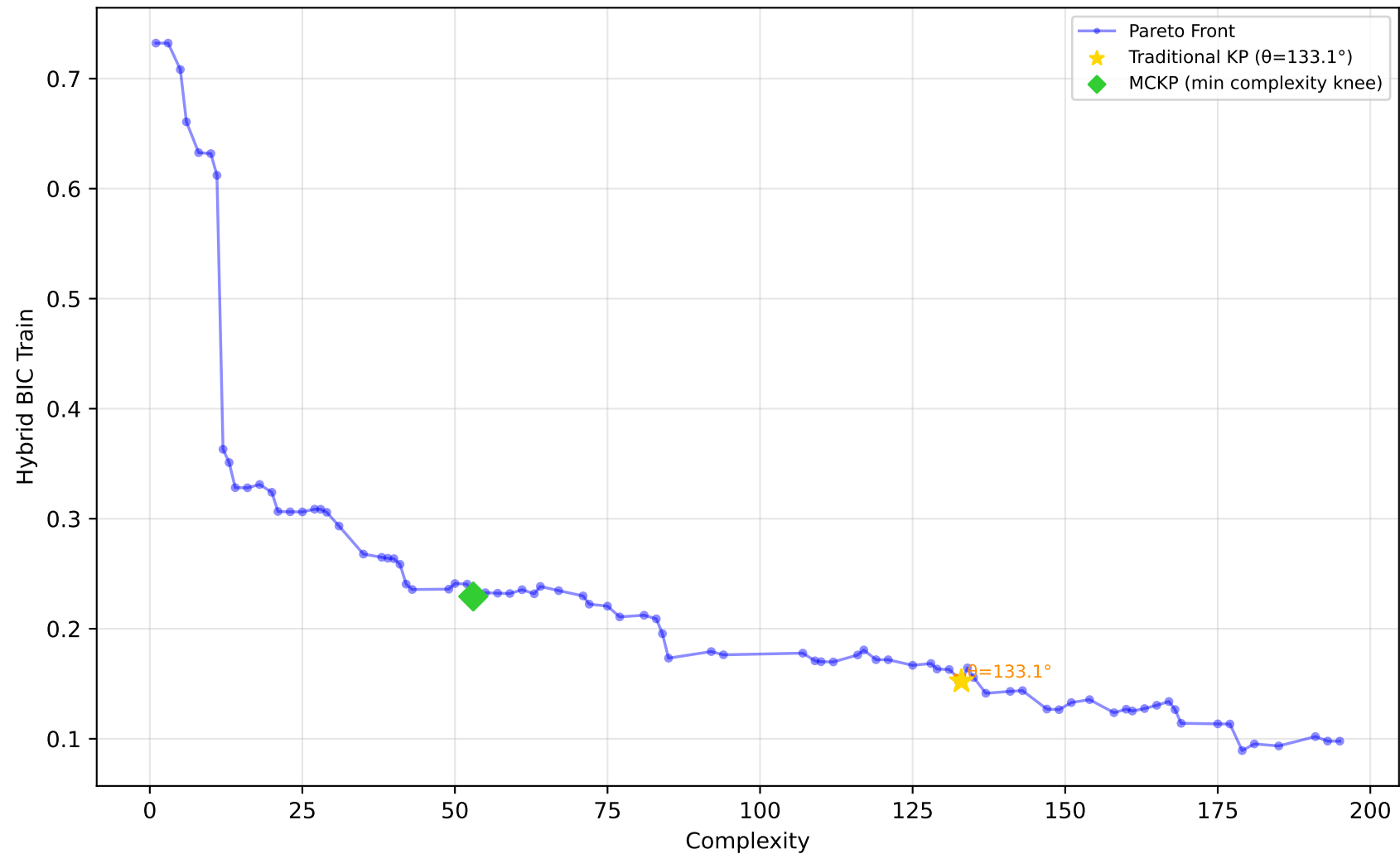
557_analcatdata_apnea1 - Run 3 - SVP - Hybrid BIC Train \lambda_1=0.00, \lambda_2=0.00, \lambda_3=0.00 | Difficulty: 0.85 | Method: hmr
