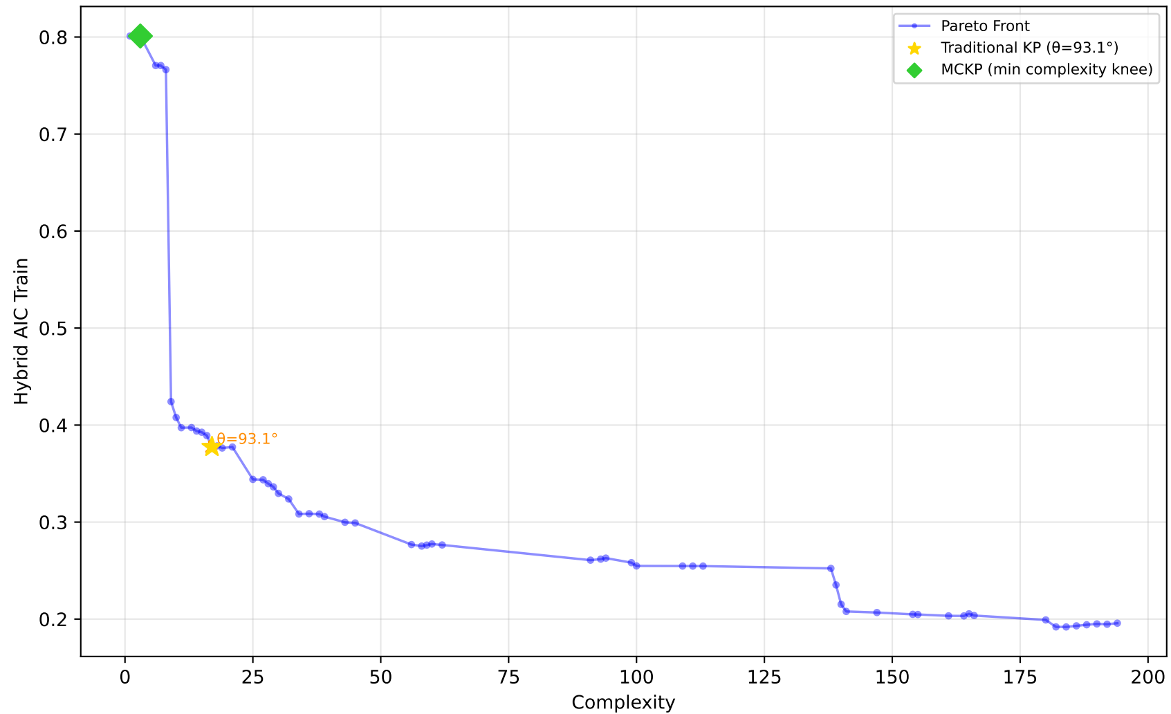
557_analcatdata_apnea1 - Run 4 - MVP - Hybrid AIC Train \lambda_1=0.00, \lambda_2=0.00, \lambda_3=0.00 | Difficulty: 1.00 | Method: hmr
