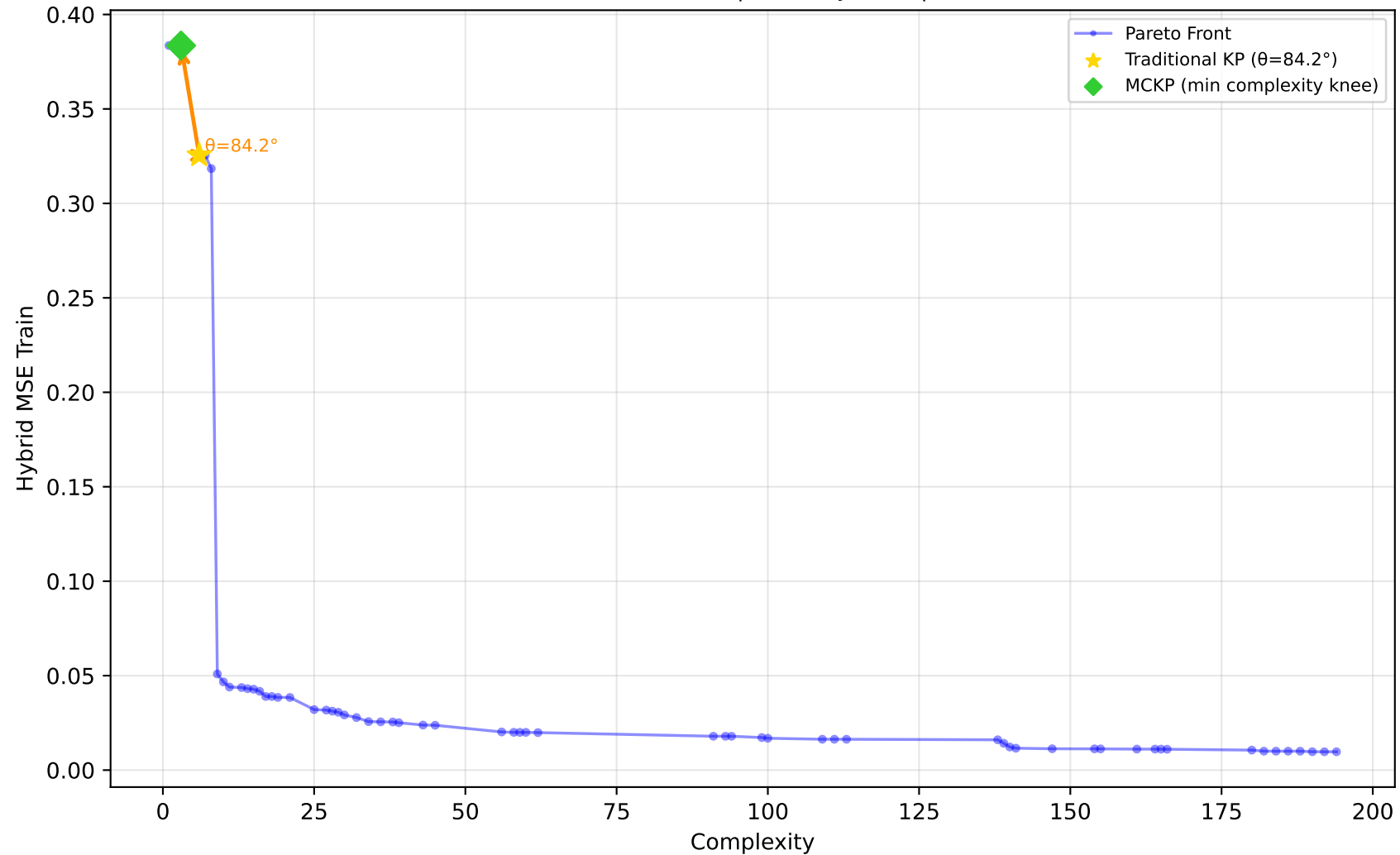
557_analcatdata_apnea1 - Run 4 - MVP - Hybrid MSE Train \lambda_1=0.00 , \lambda_2=0.00 , \lambda_3=0.00 | Difficulty: 1.00 | Method: hmr
