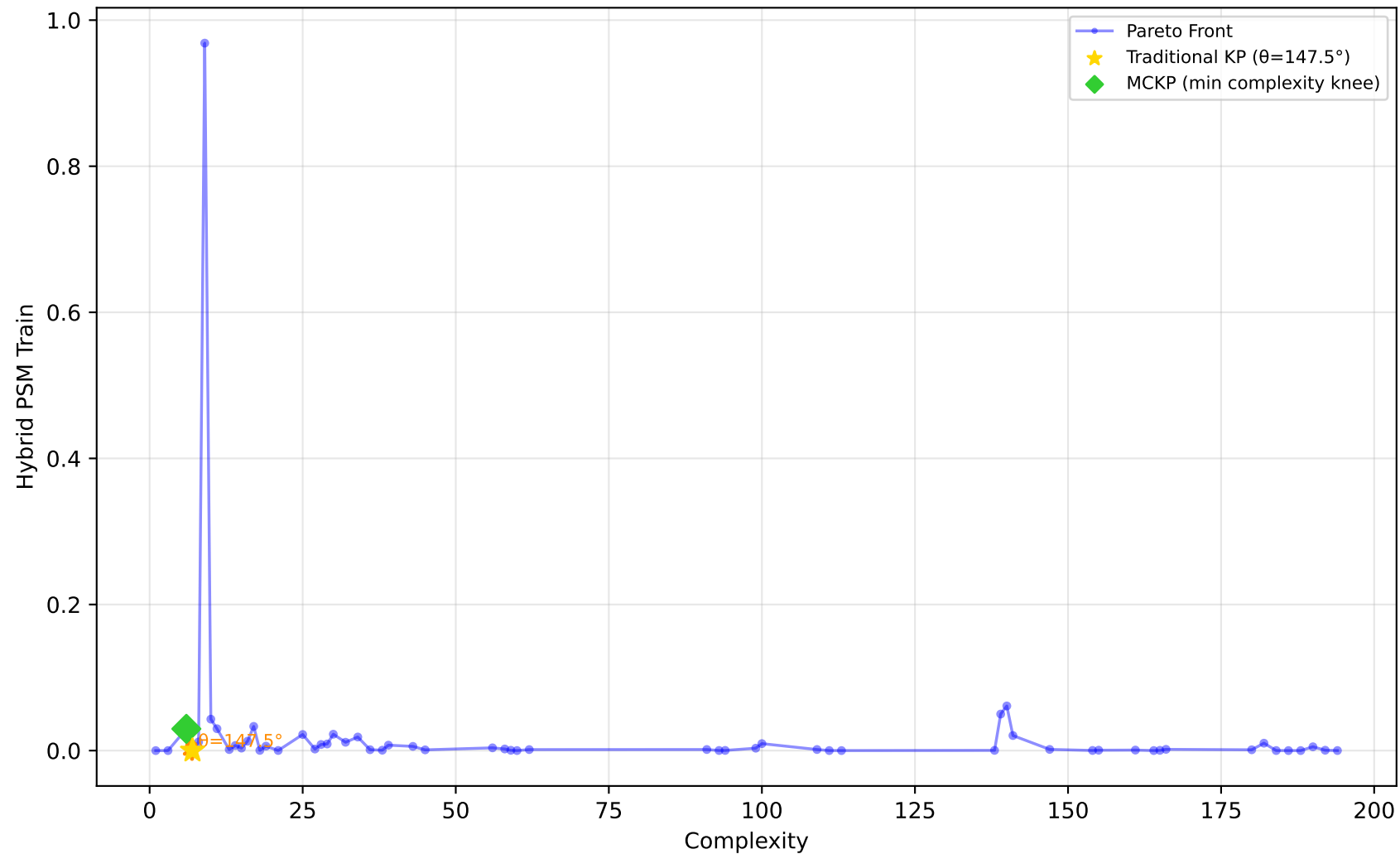
557_analcatdata_apnea1 - Run 4 - MVP - Hybrid PSM Train \lambda_1=0.00, \lambda_2=0.00, \lambda_3=0.00 | Difficulty: 1.00 | Method: hmr
