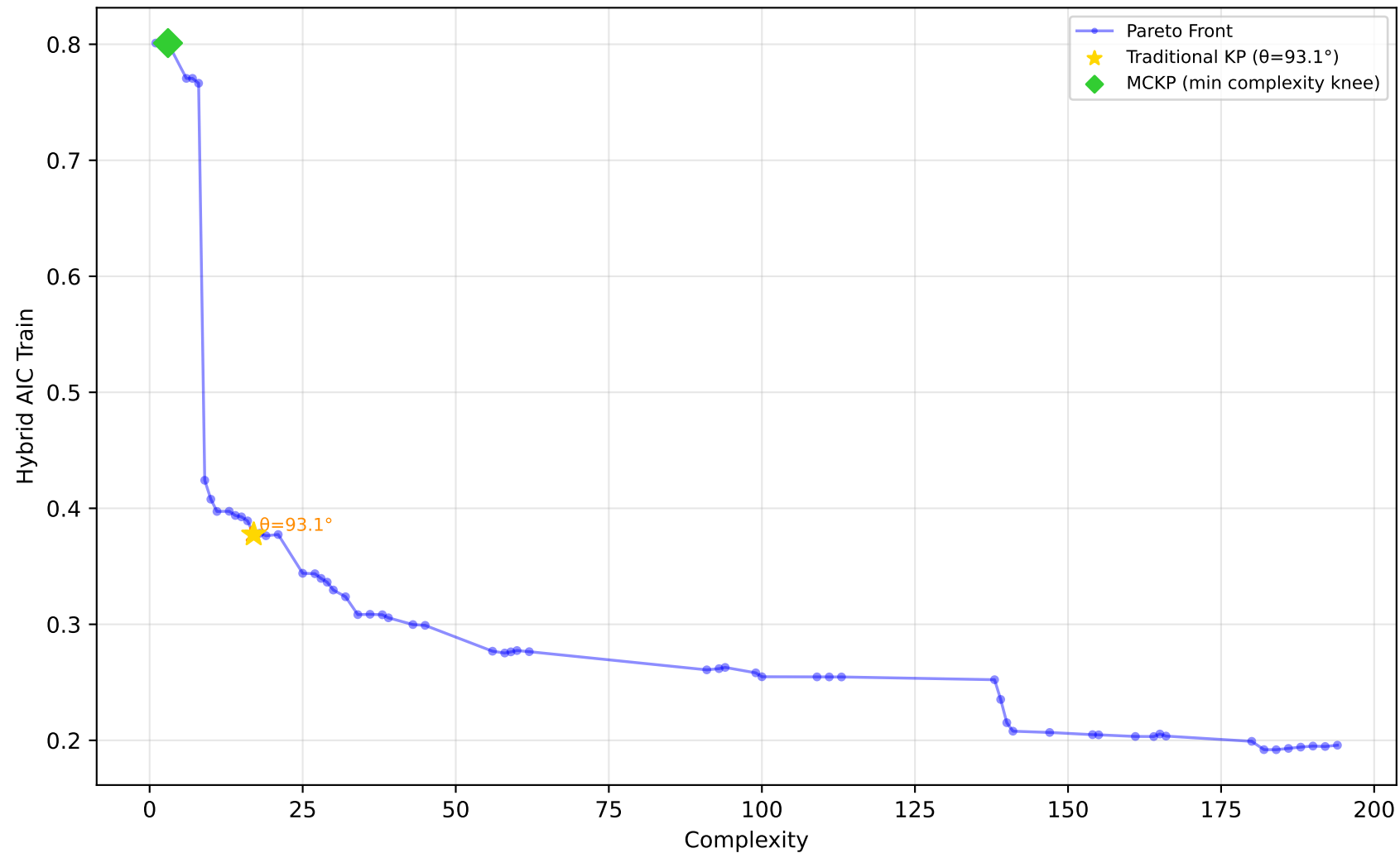
557_analcatdata_apnea1 - Run 4 - SVP - Hybrid AIC Train \lambda_1=0.00, \lambda_2=0.00, \lambda_3=0.00 | Difficulty: 1.00 | Method: hmr
