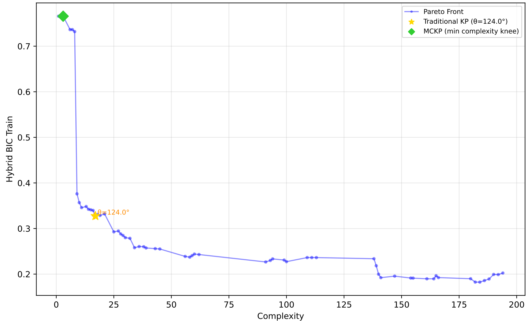
557_analcatdata_apnea1 - Run 4 - SVP - Hybrid BIC Train \lambda_1=0.00, \lambda_2=0.00, \lambda_3=0.00 | Difficulty: 1.00 | Method: hmr
