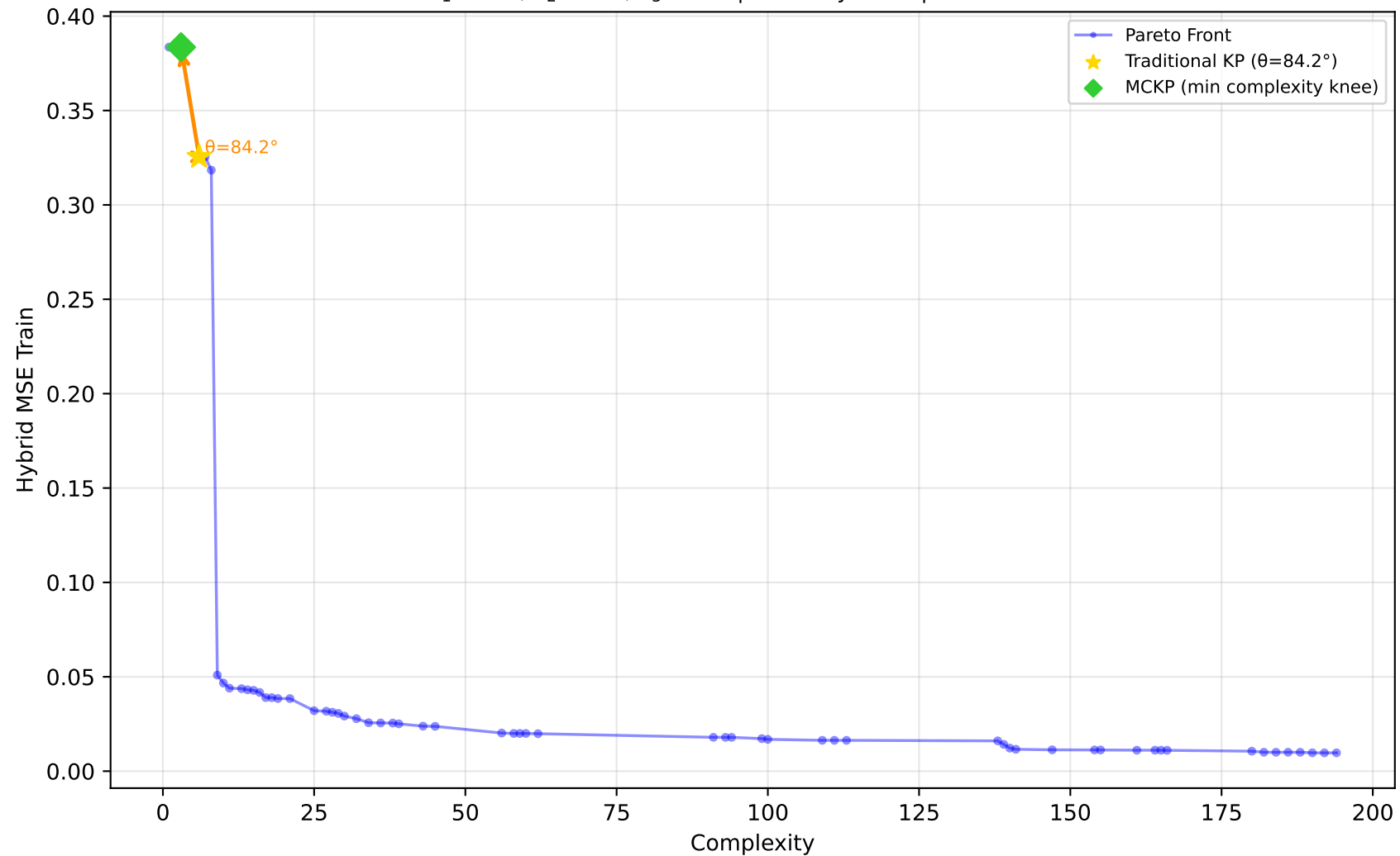
557_analcatdata_apnea1 - Run 4 - SVP - Hybrid MSE Train \lambda_1=0.00 , \lambda_2=0.00 , \lambda_3=0.00 | Difficulty: 1.00 | Method: hmr
