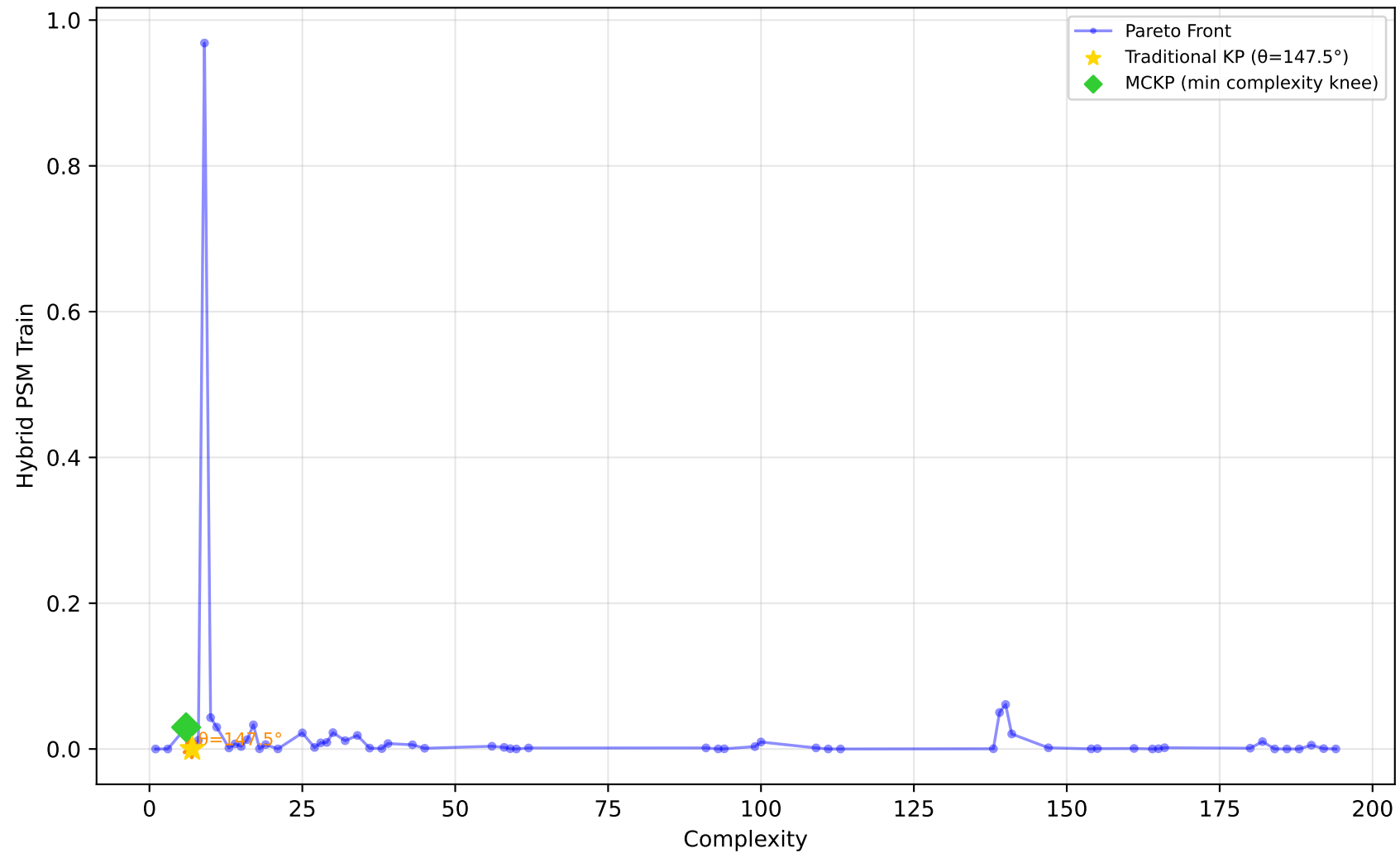
557_analcatdata_apnea1 - Run 4 - SVP - Hybrid PSM Train \lambda_1=0.00, \lambda_2=0.00, \lambda_3=0.00 | Difficulty: 1.00 | Method: hmr
