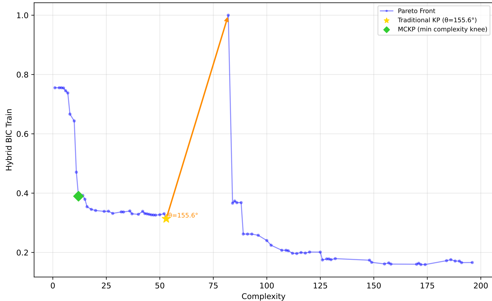
557_analcatdata_apnea1 - Run 5 - MVP - Hybrid BIC Train \lambda_1=0.00, \lambda_2=0.00, \lambda_3=0.00 | Difficulty: 0.94 | Method: hmr
