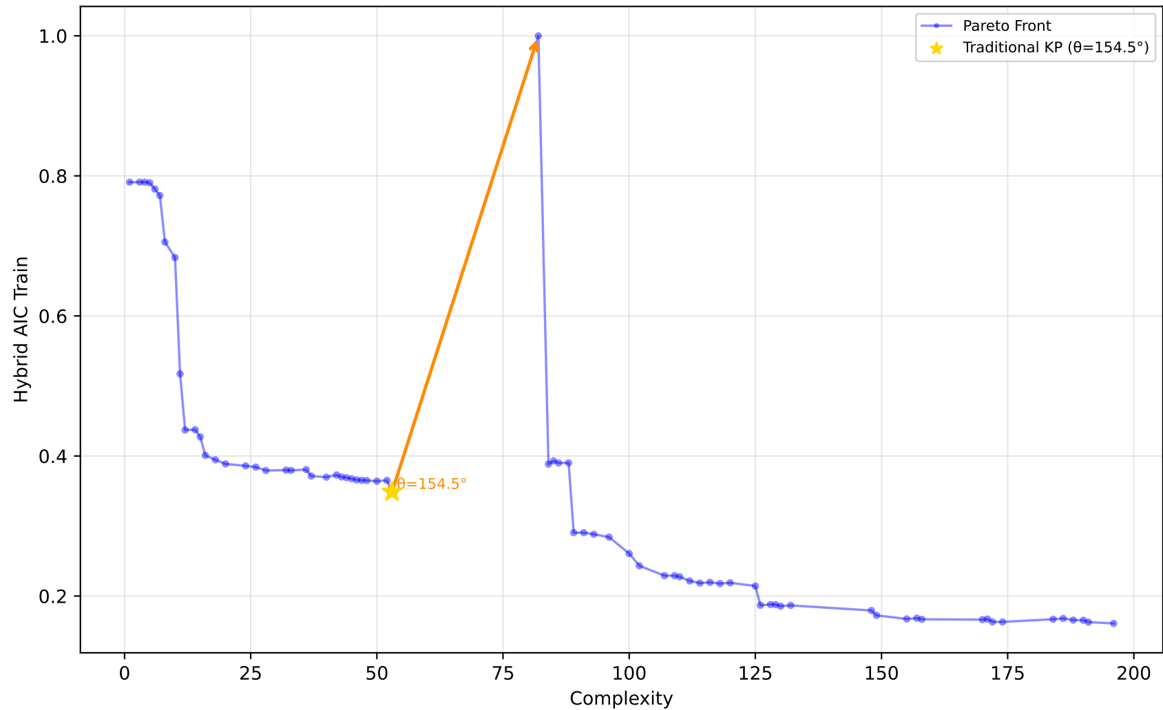
557_analcatdata_apnea1 - Run 5 - SVP - Hybrid AIC Train \lambda_1=0.00, \lambda_2=0.00, \lambda_3=0.00 | Difficulty: 0.94 | Method: hmr
