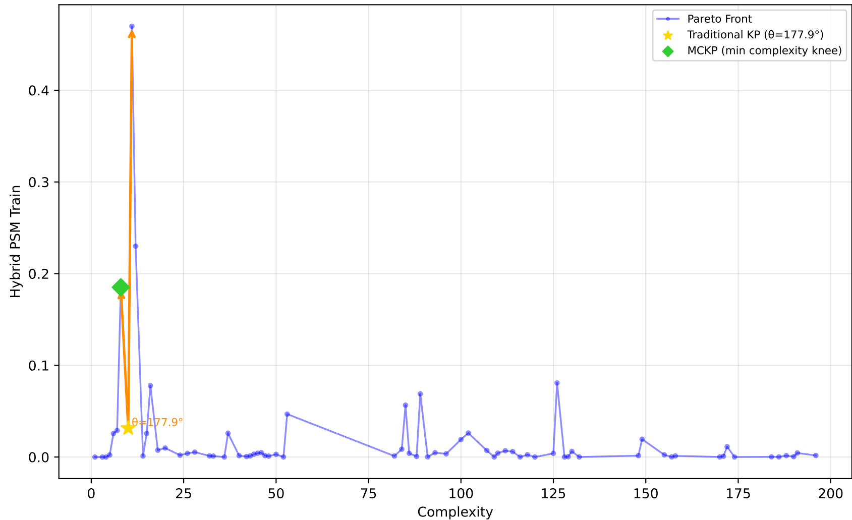
557_analcatdata_apnea1 - Run 5 - SVP - Hybrid PSM Train \lambda_1=0.00, \lambda_2=0.00, \lambda_3=0.00 | Difficulty: 0.94 | Method: hmr
