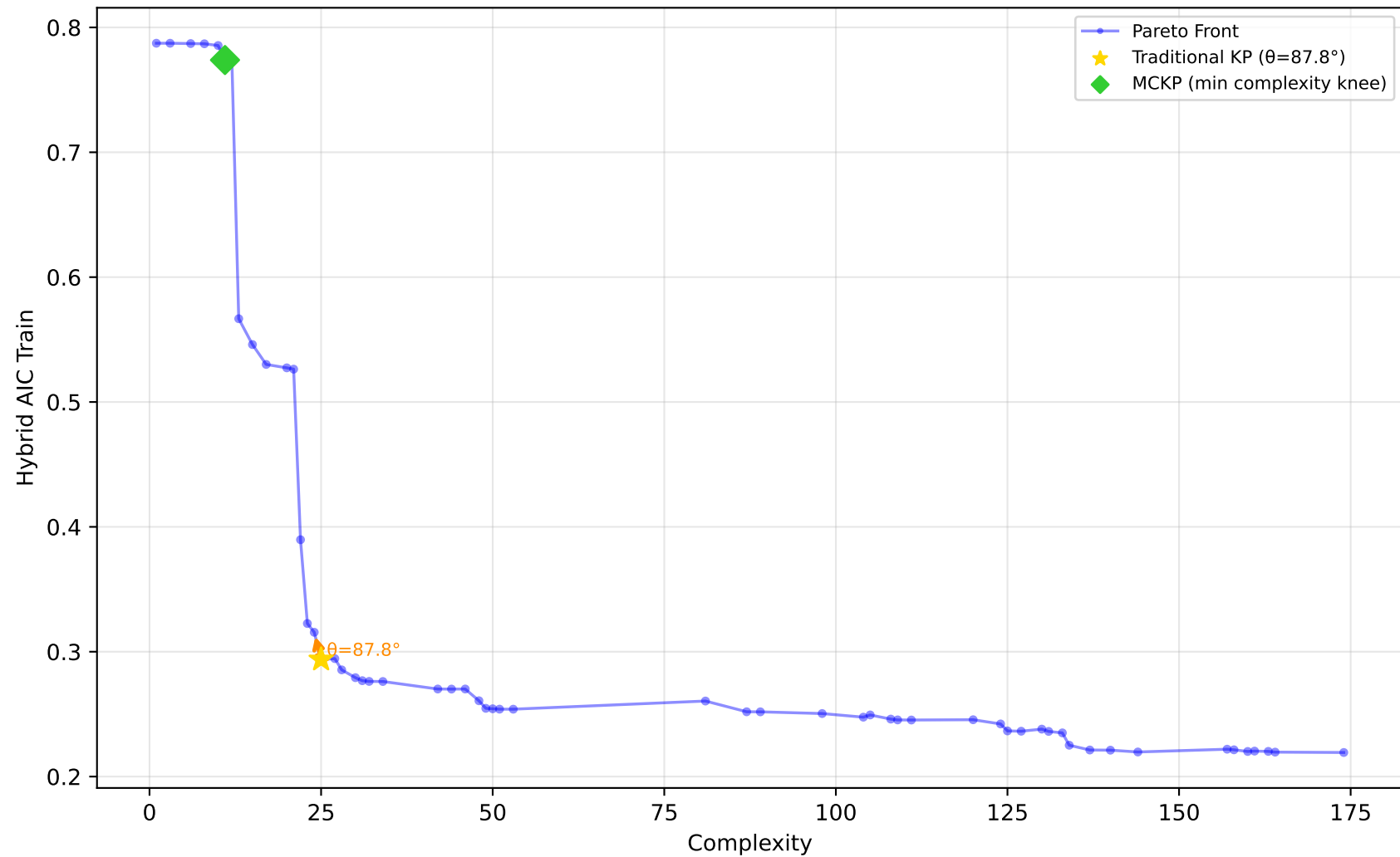
557_analcatdata_apnea1 - Run 6 - SVP - Hybrid AIC Train \lambda_1=0.00, \lambda_2=0.00, \lambda_3=0.00 | Difficulty: 1.00 | Method: hmr
