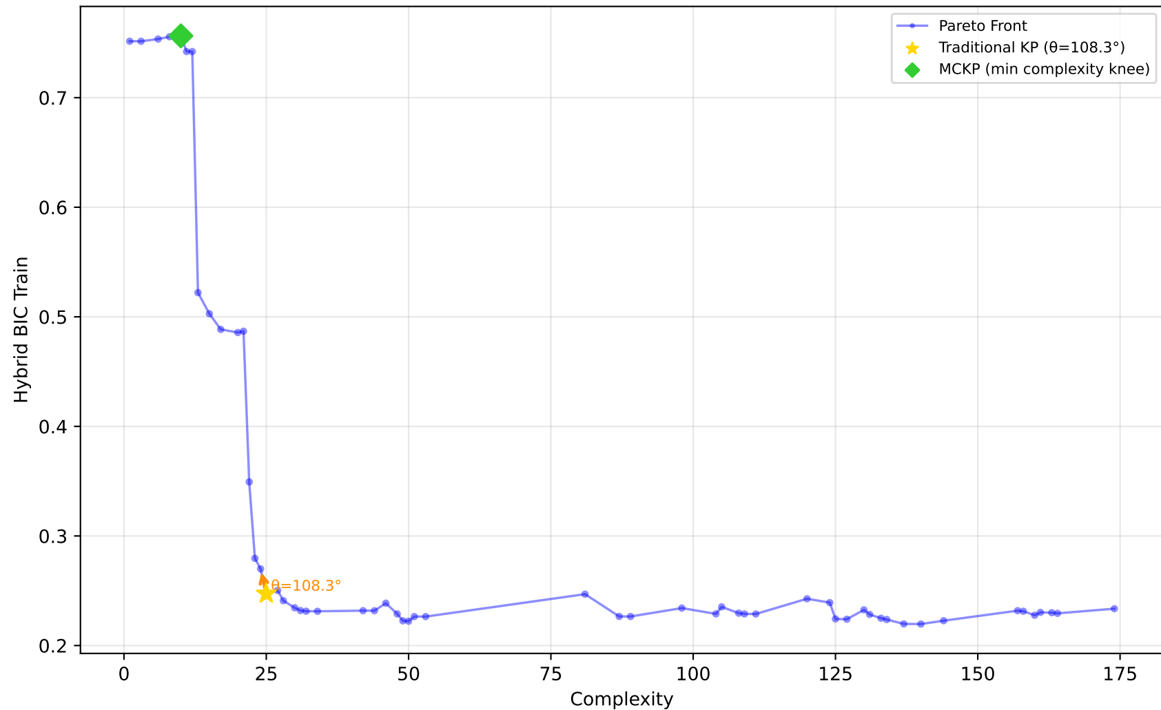
557_analcatdata_apnea1 - Run 6 - SVP - Hybrid BIC Train \lambda_1=0.00, \lambda_2=0.00, \lambda_3=0.00 | Difficulty: 1.00 | Method: hmr
