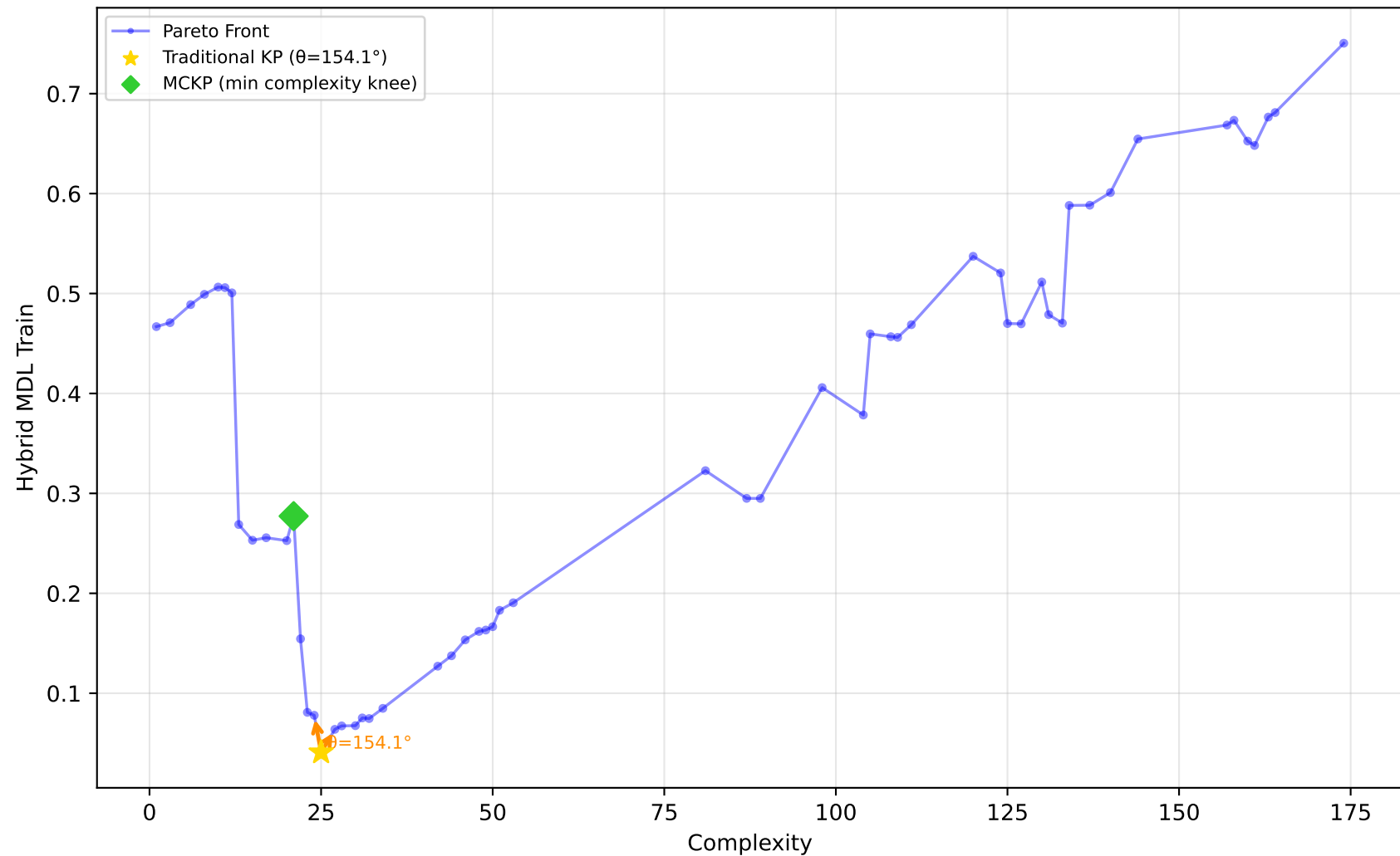
557_analcatdata_apnea1 - Run 6 - SVP - Hybrid MDL Train \lambda_1=0.00, \lambda_2=0.00, \lambda_3=0.00 | Difficulty: 1.00 | Method: hmr
