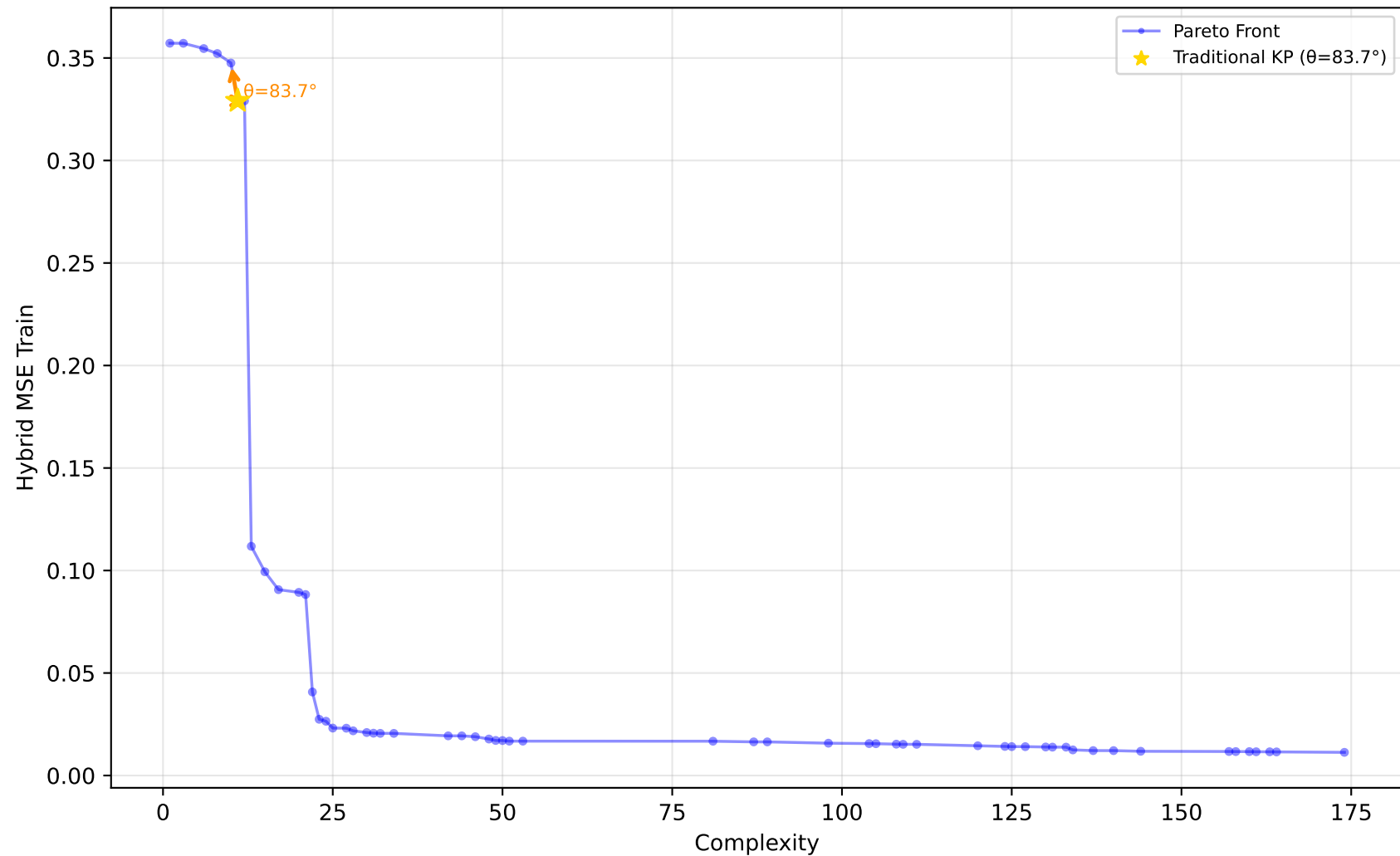
557_analcatdata_apnea1 - Run 6 - SVP - Hybrid MSE Train \lambda_1=0.00, \lambda_2=0.00, \lambda_3=0.00 | Difficulty: 1.00 | Method: hmr
