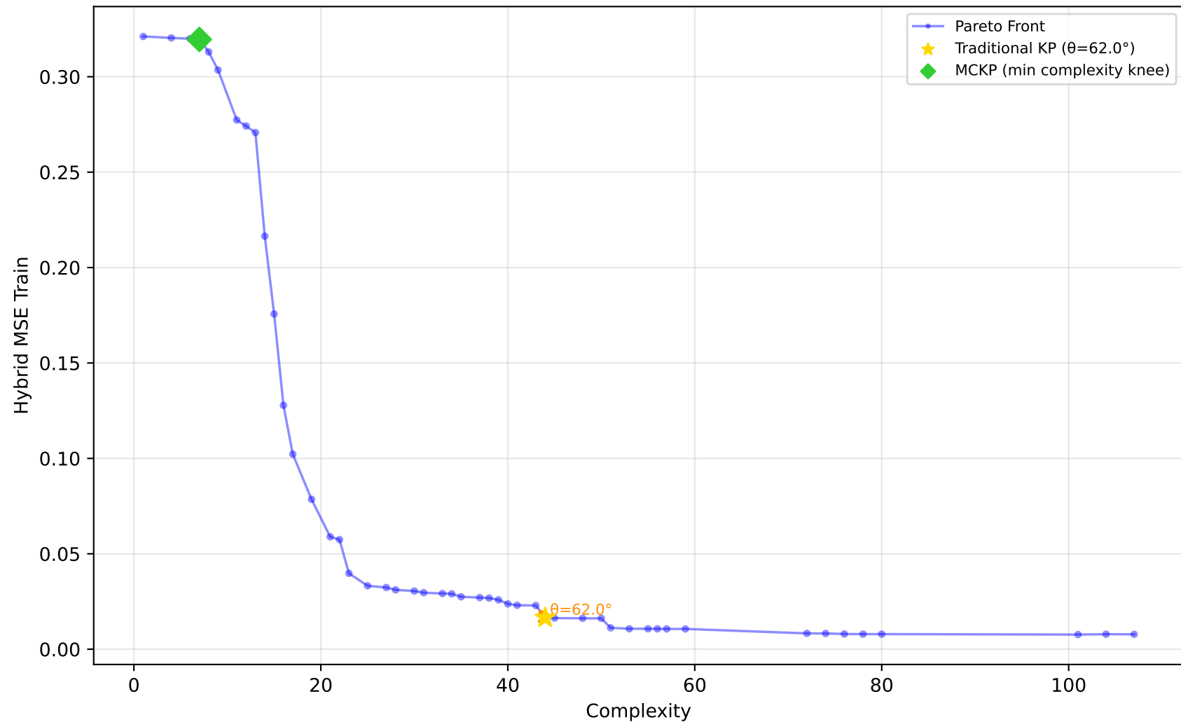
557_analcatdata_apnea1 - Run 7 - SVP - Hybrid MSE Train \lambda_1=0.00, \lambda_2=0.00, \lambda_3=0.00 | Difficulty: 1.00 | Method: hmr
