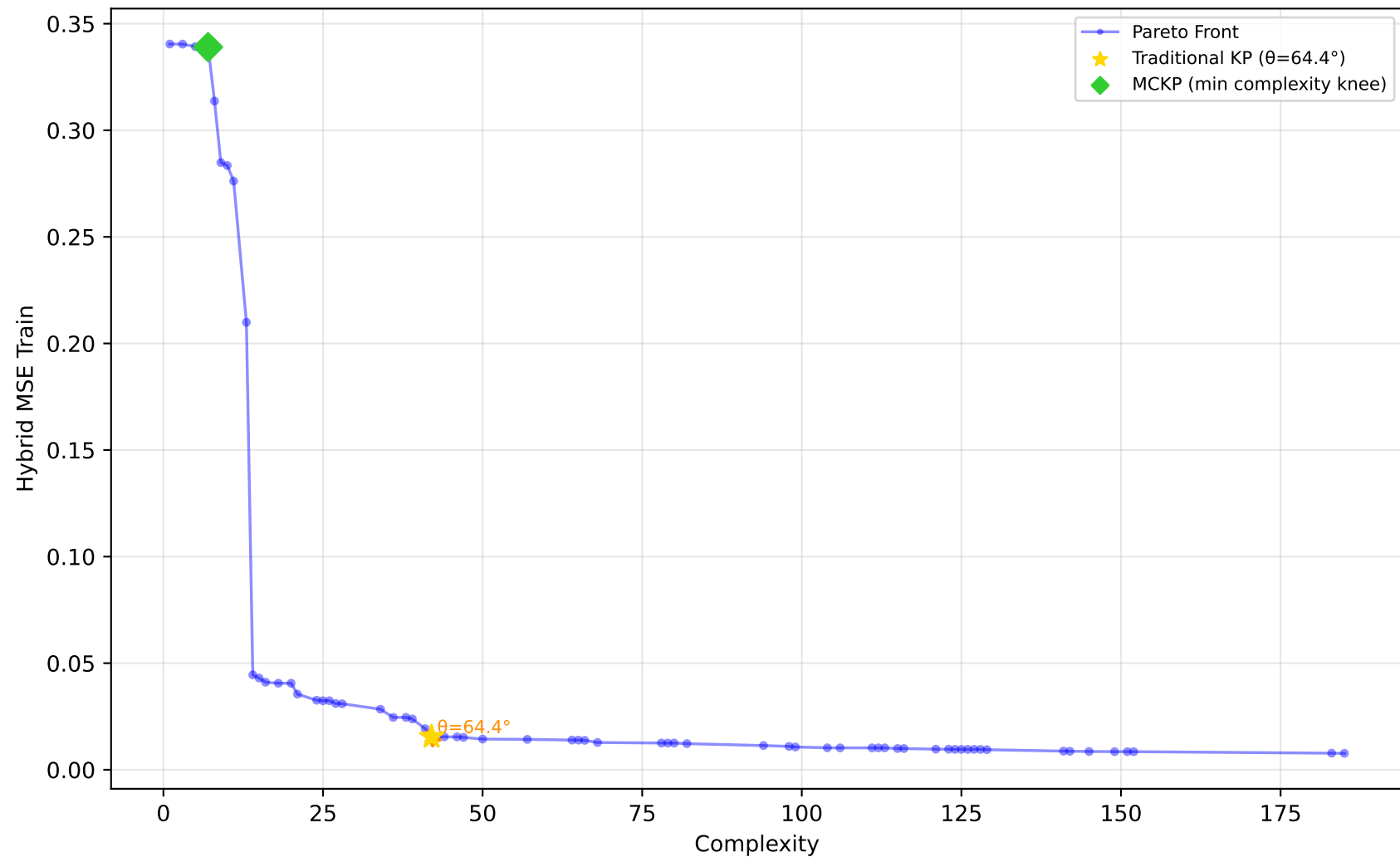
557_analcatdata_apnea1 - Run 8 - MVP - Hybrid MSE Train \lambda_1=0.00 , \lambda_2=0.00 , \lambda_3=0.00 | Difficulty: 1.00 | Method: hmr
