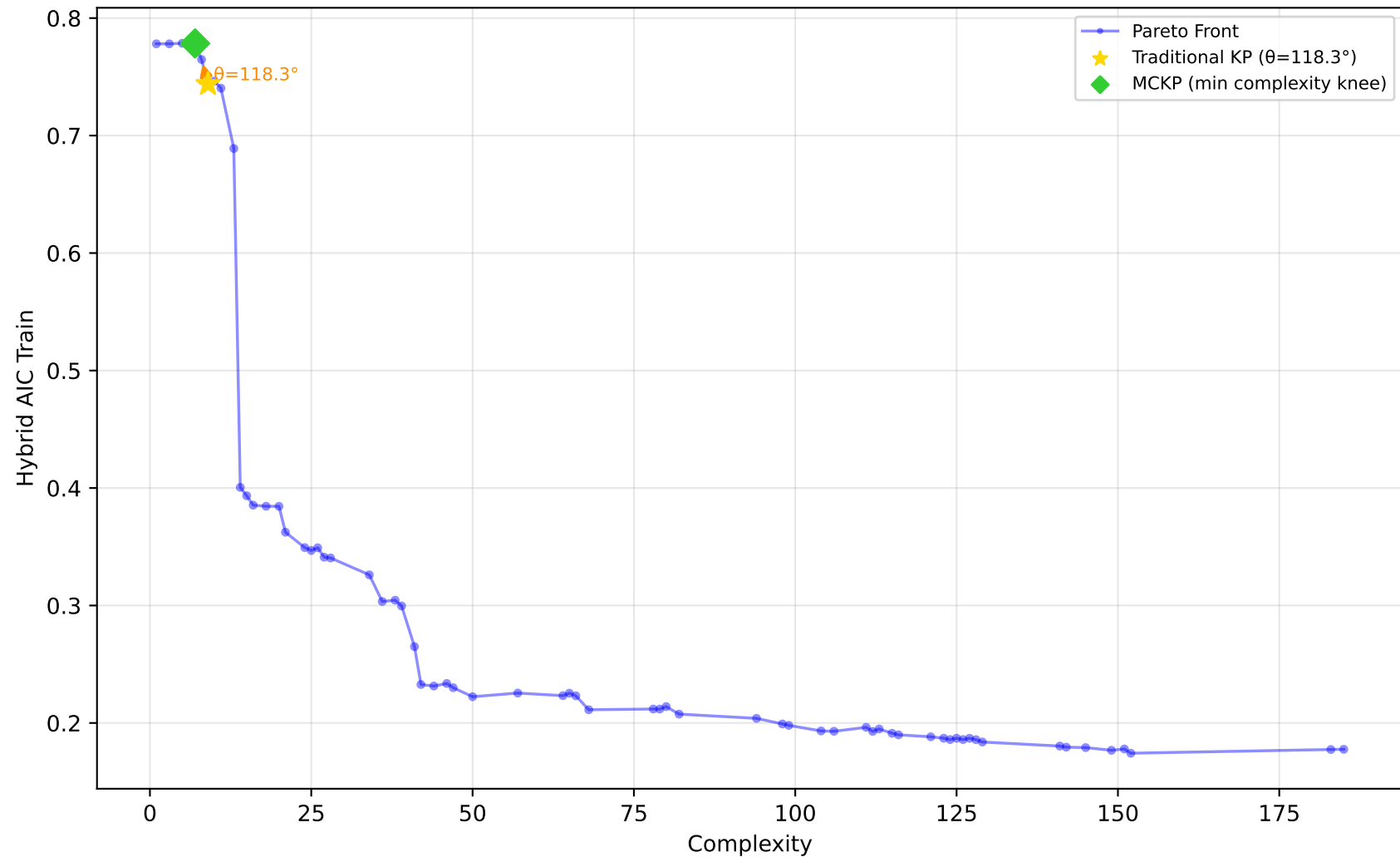
557_analcatdata_apnea1 - Run 8 - SVP - Hybrid AIC Train \lambda_1=0.00, \lambda_2=0.00, \lambda_3=0.00 | Difficulty: 1.00 | Method: hmr
