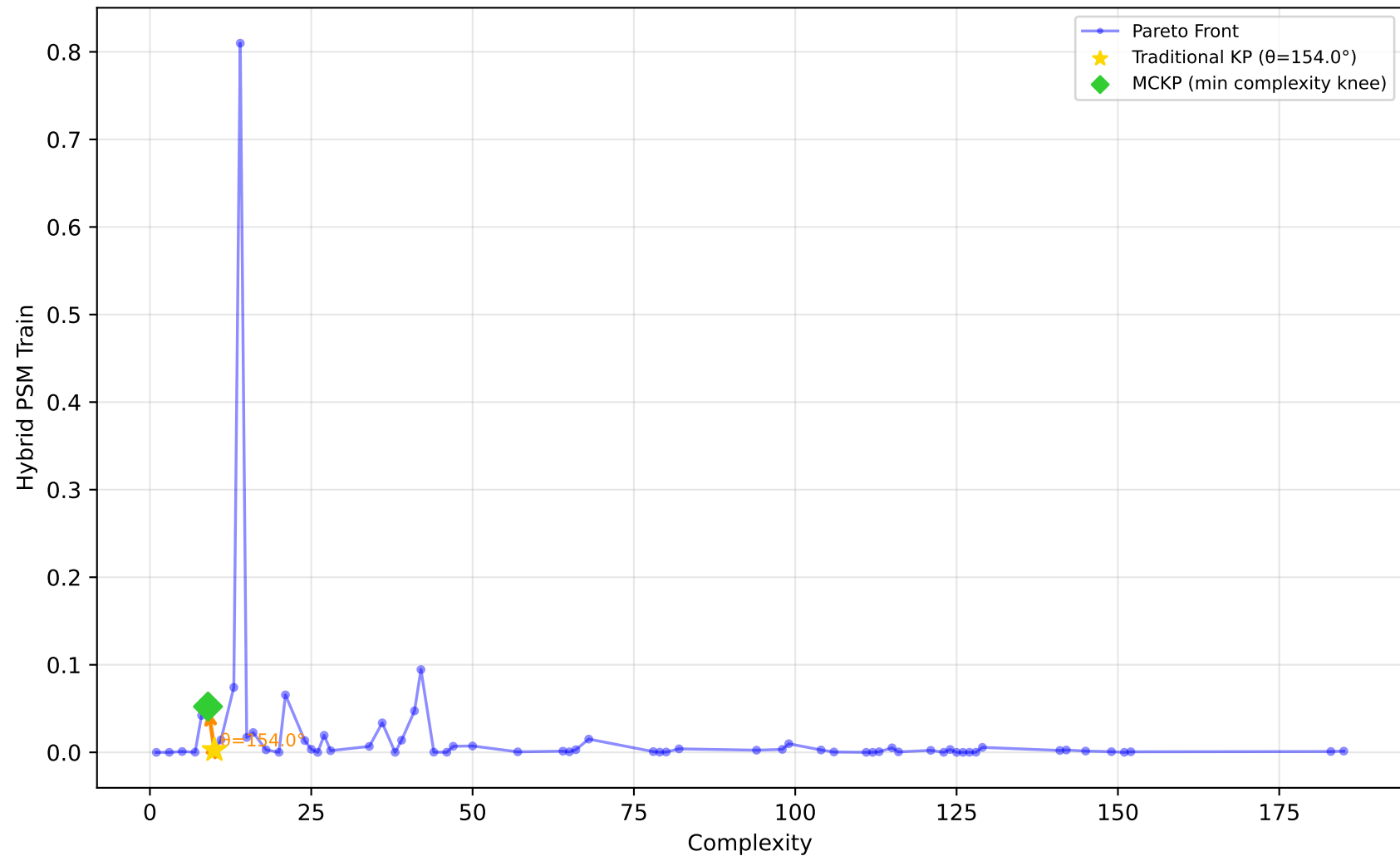
557_analcatdata_apnea1 - Run 8 - SVP - Hybrid PSM Train \lambda_1=0.00, \lambda_2=0.00, \lambda_3=0.00 | Difficulty: 1.00 | Method: hmr
