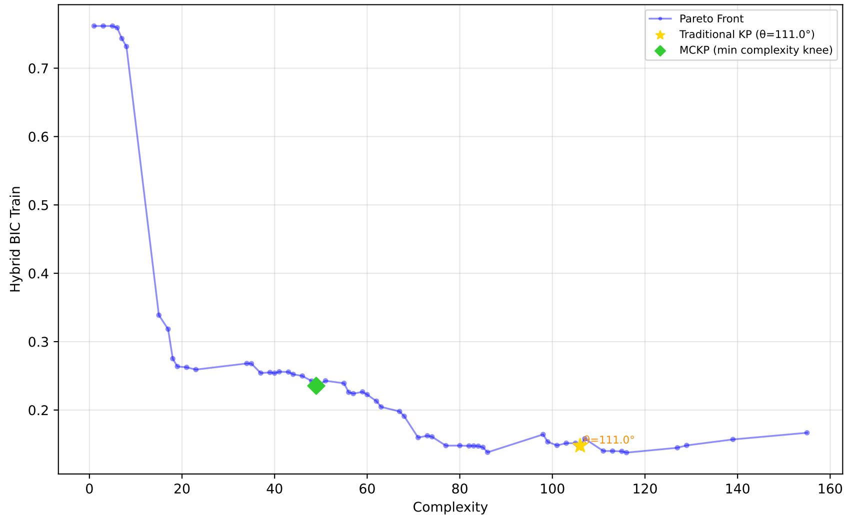
557_analcatdata_apnea1 - Run 9 - MVP - Hybrid BIC Train \lambda_1=0.00, \lambda_2=0.00, \lambda_3=0.00 | Difficulty: 1.00 | Method: hmr
