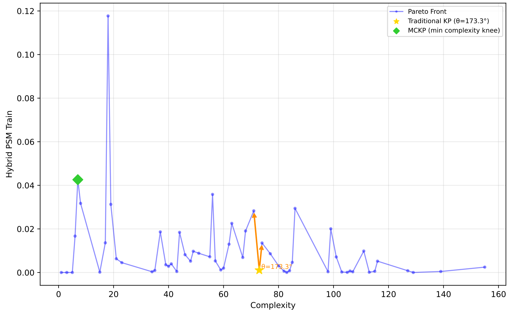
557_analcatdata_apnea1 - Run 9 - MVP - Hybrid PSM Train \lambda_1=0.00 , \lambda_2=0.00 , \lambda_3=0.00 | Difficulty: 1.00 | Method: hmr
