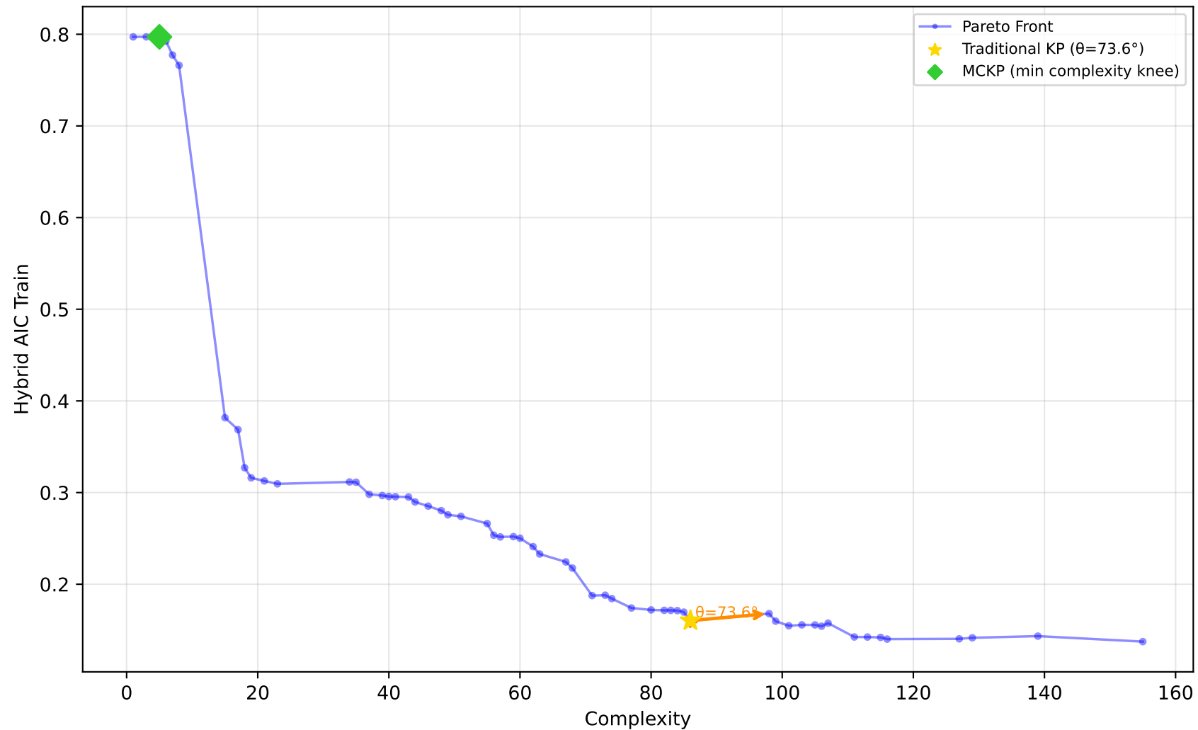
557_analcatdata_apnea1 - Run 9 - SVP - Hybrid AIC Train \lambda_1=0.00, \lambda_2=0.00, \lambda_3=0.00 | Difficulty: 1.00 | Method: hmr
