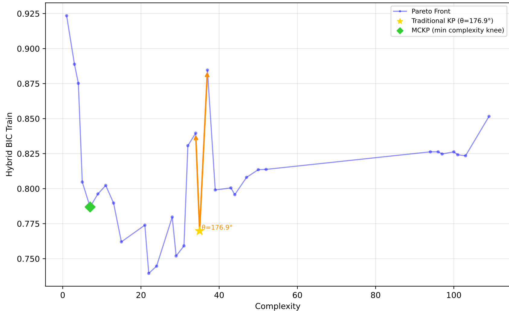
1096_FacultySalaries - Run 10 - MVP - Hybrid BIC Train \lambda_1=0.10 , \lambda_2=0.00 , \lambda_3=0.00 | Difficulty: 1.00 | Method: hmr
