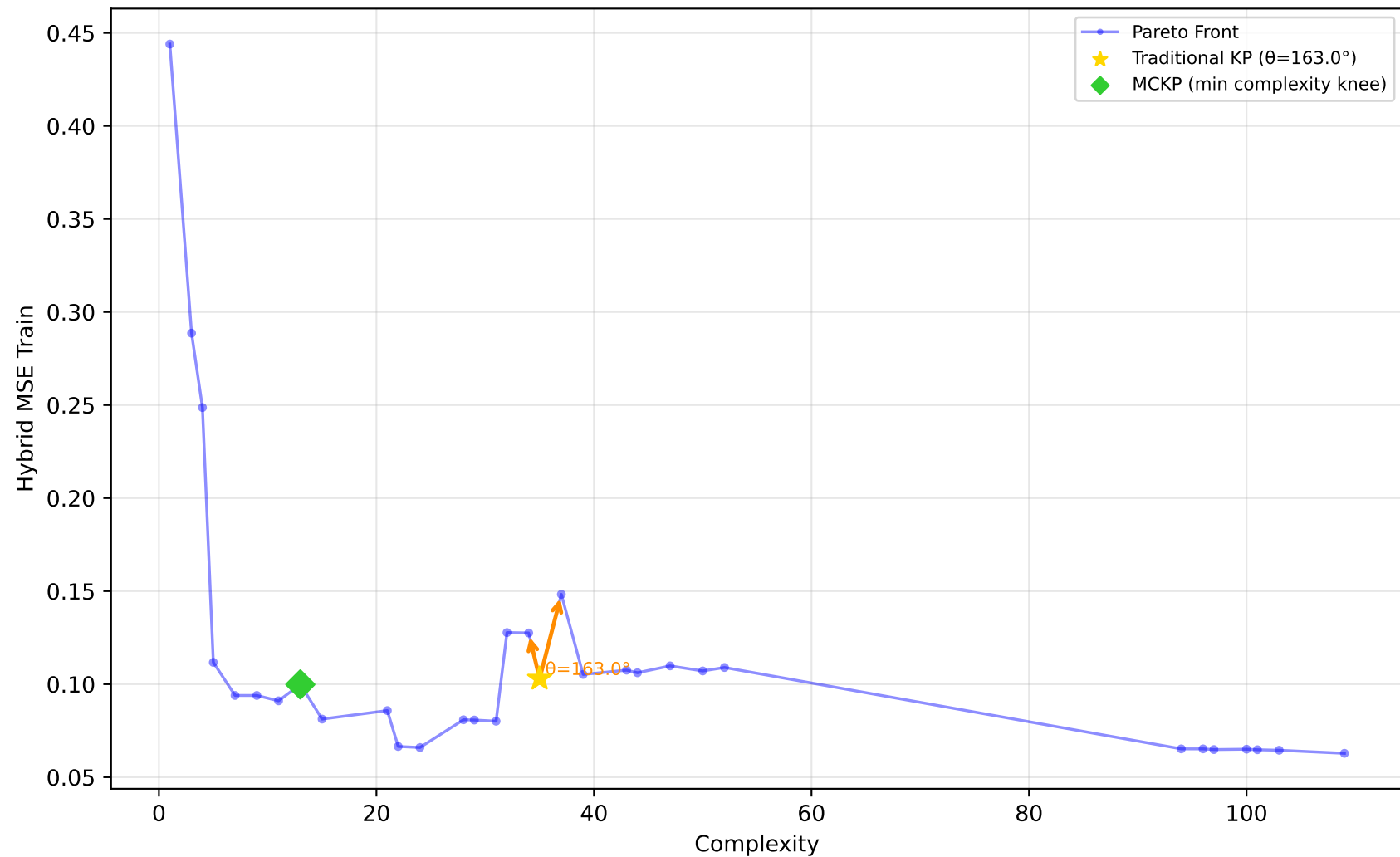
1096_FacultySalaries - Run 10 - MVP - Hybrid MSE Train \lambda_1=0.10 , \lambda_2=0.00 , \lambda_3=0.00 | Difficulty: 1.00 | Method: hmr
