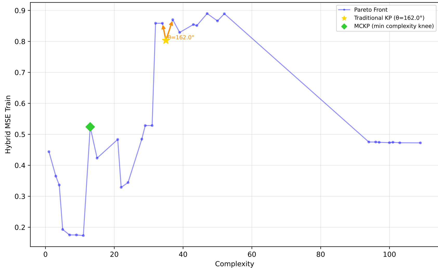
1096_FacultySalaries - Run 10 - MVP - Hybrid MSE Train \lambda_1=1.00, \lambda_2=0.00, \lambda_3=0.00 | Difficulty: 1.00 | Method: hmr
