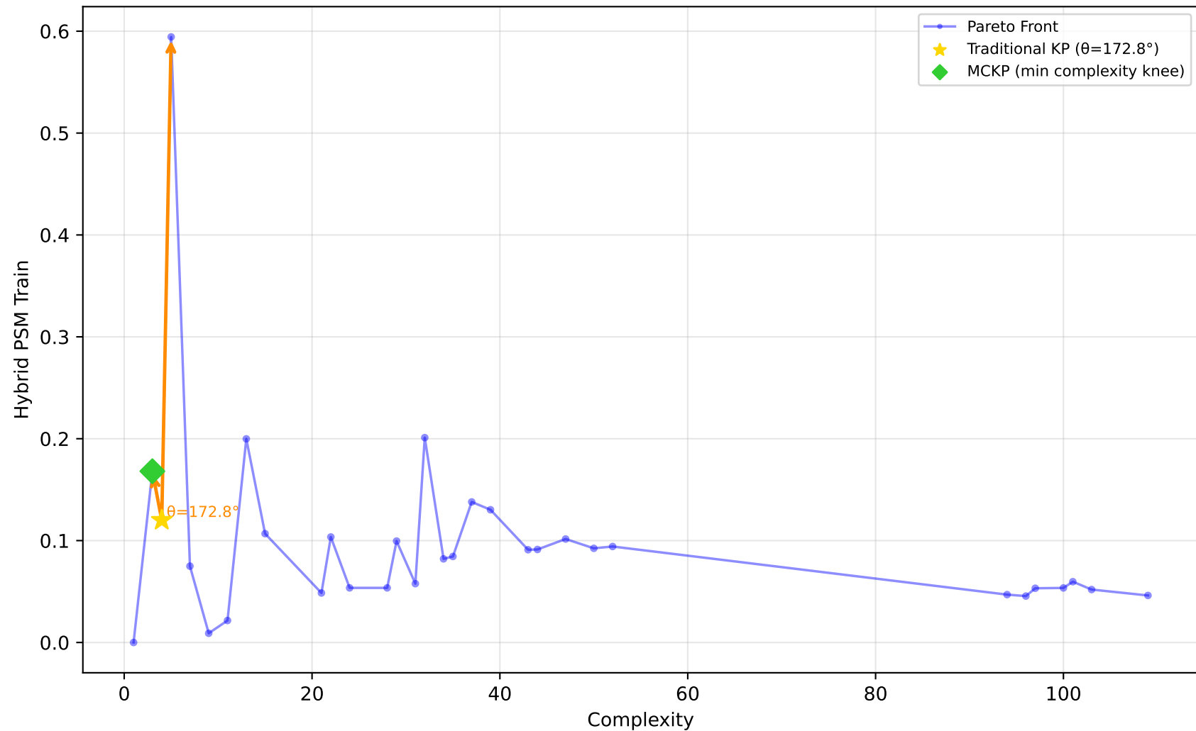
1096_FacultySalaries - Run 10 - MVP - Hybrid PSM Train \lambda_1=0.10 , \lambda_2=0.00 , \lambda_3=0.00 | Difficulty: 1.00 | Method: hmr
