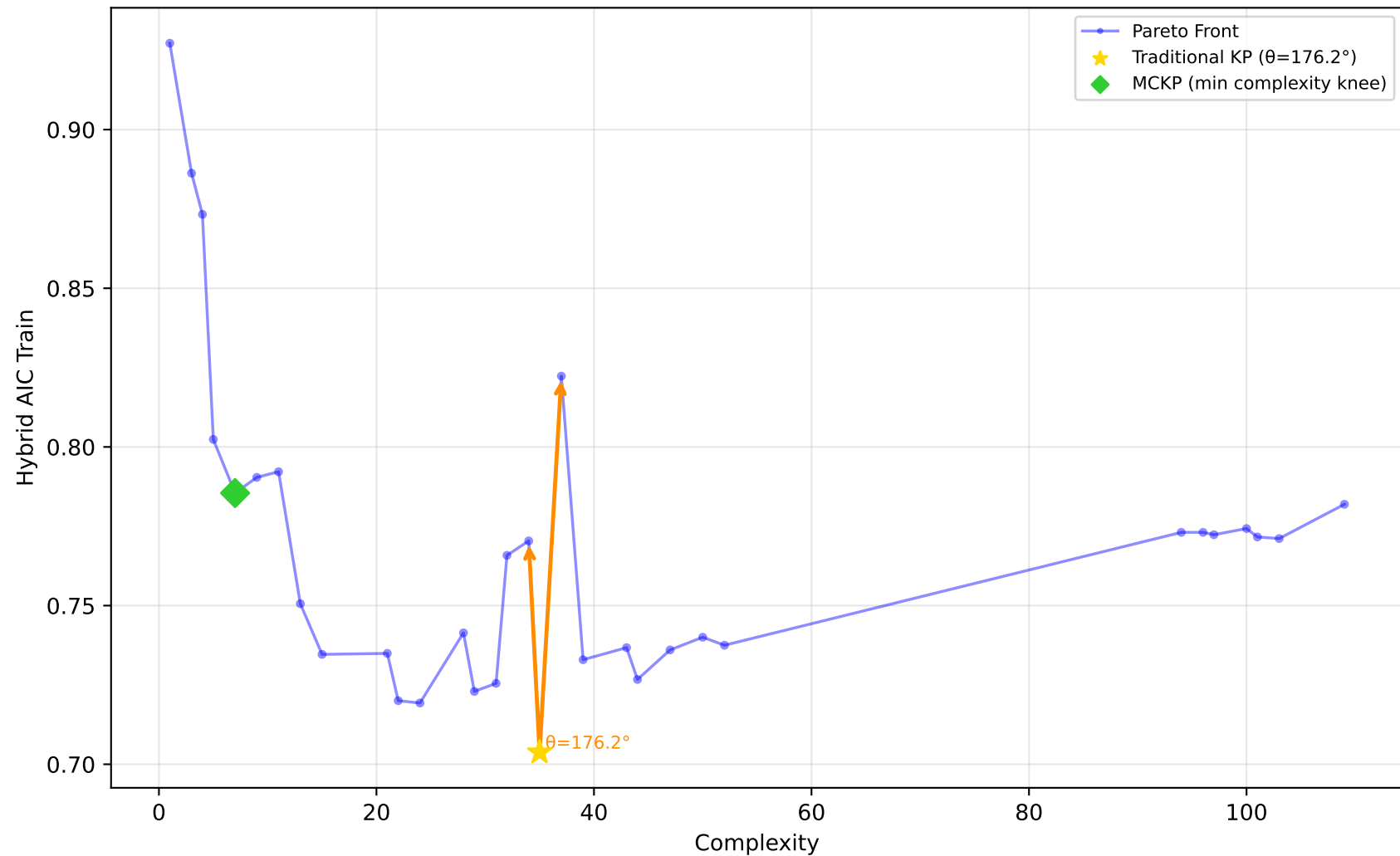
1096_FacultySalaries - Run 10 - SVP - Hybrid AIC Train \lambda_1=0.00 , \lambda_2=0.90 , \lambda_3=0.00 | Difficulty: 1.00 | Method: hmr
