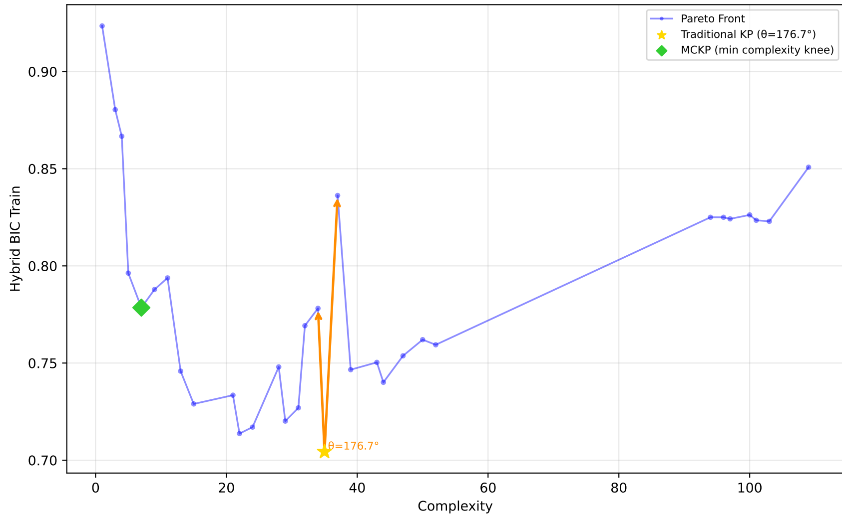
1096_FacultySalaries - Run 10 - SVP - Hybrid BIC Train \lambda_1=0.00 , \lambda_2=0.90 , \lambda_3=0.00 | Difficulty: 1.00 | Method: hmr
