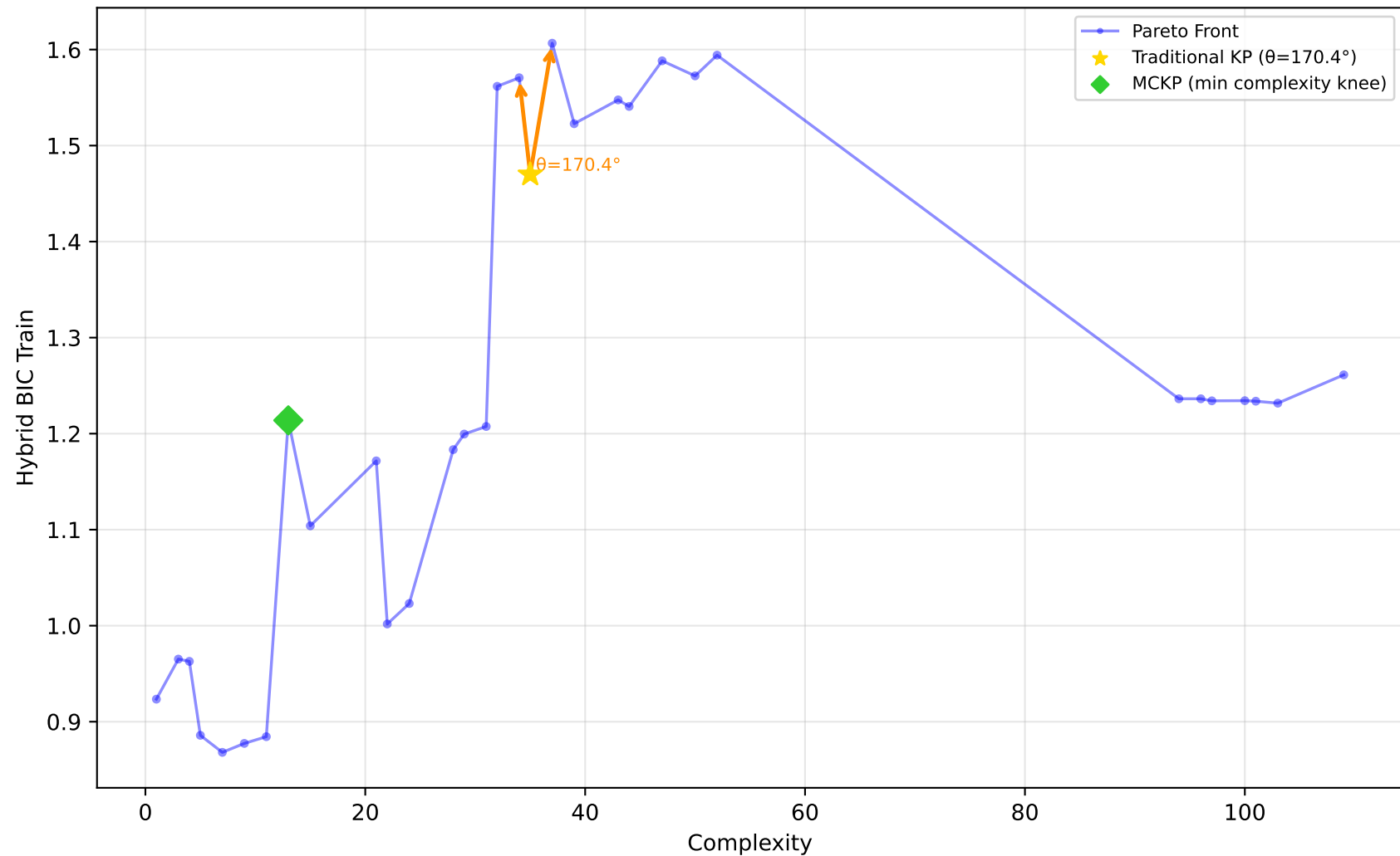
1096_FacultySalaries - Run 10 - SVP - Hybrid BIC Train \lambda_1=1.00 , \lambda_2=0.00 , \lambda_3=0.00 | Difficulty: 1.00 | Method: hmr
