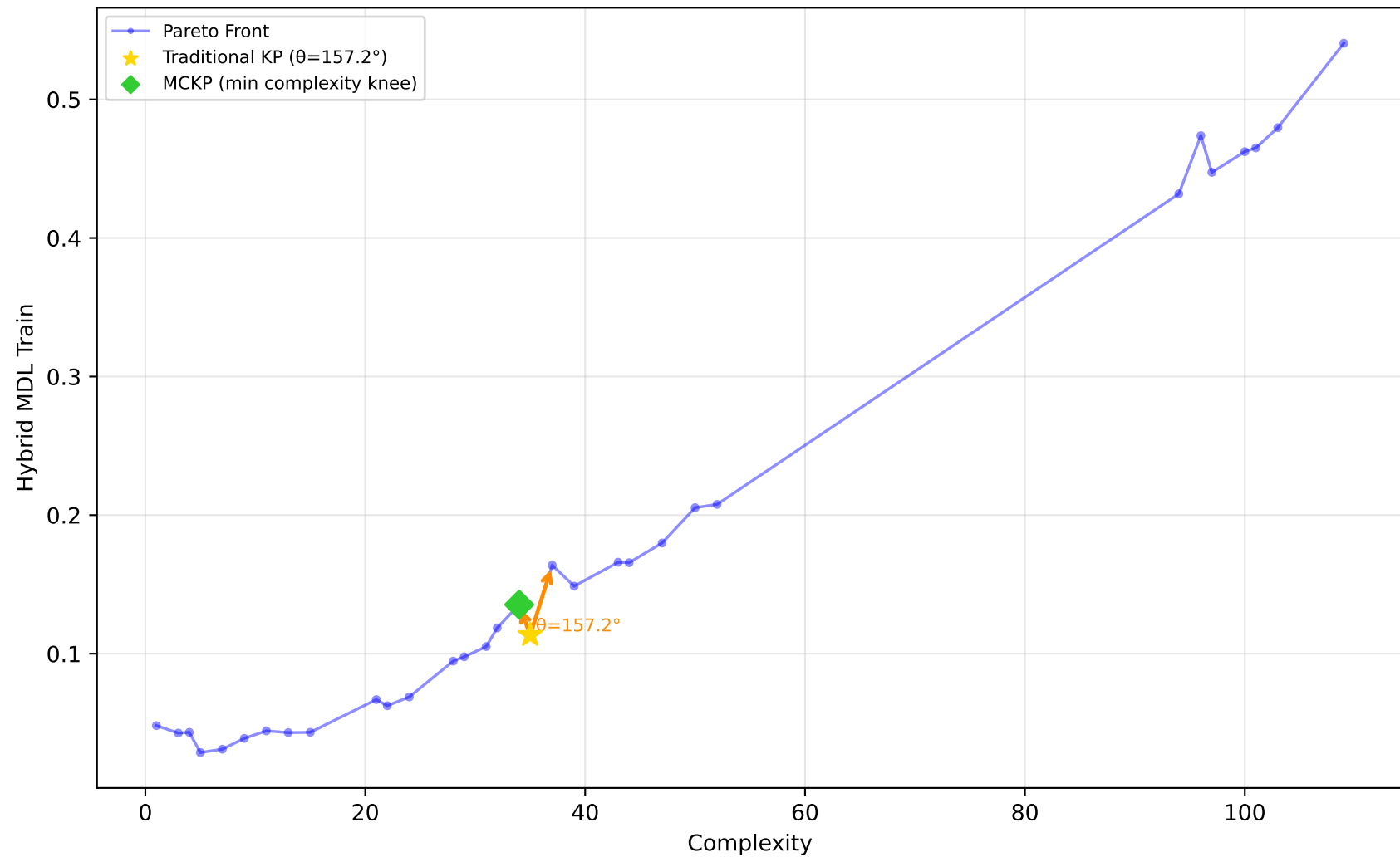
1096_FacultySalaries - Run 10 - SVP - Hybrid MDL Train \lambda_1=0.00, \lambda_2=0.90, \lambda_3=0.00 | Difficulty: 1.00 | Method: hmr
