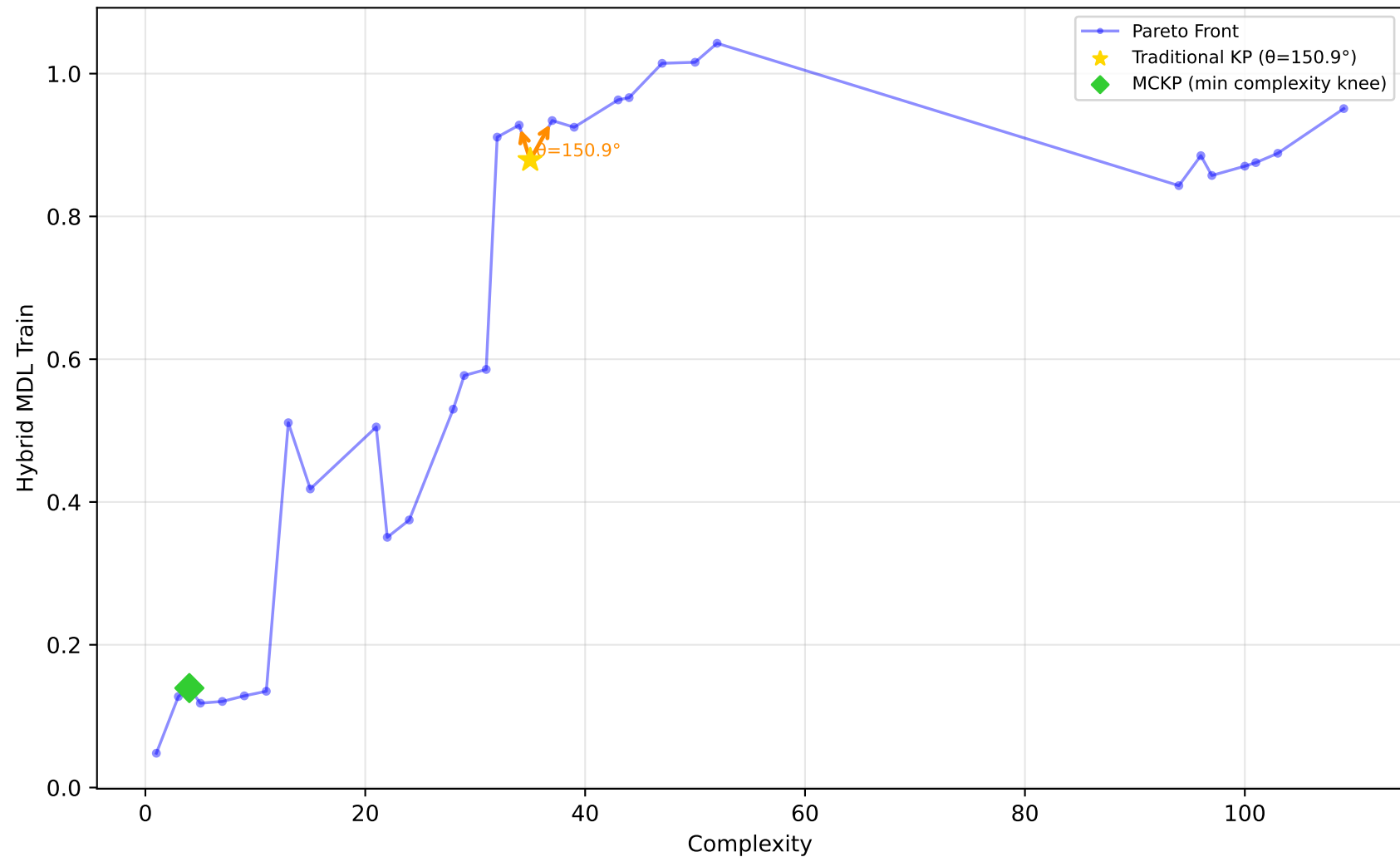
1096_FacultySalaries - Run 10 - SVP - Hybrid MDL Train \lambda_1=1.00, \lambda_2=0.00, \lambda_3=0.00 | Difficulty: 1.00 | Method: hmr
