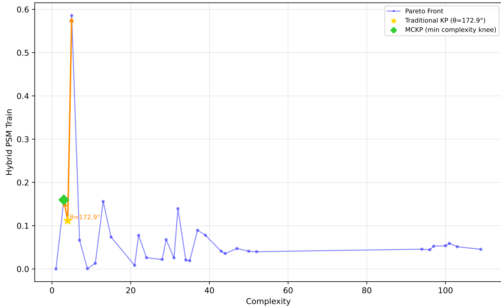
1096_FacultySalaries - Run 10 - SVP - Hybrid PSM Train \lambda_1=0.00, \lambda_2=0.90, \lambda_3=0.00 | Difficulty: 1.00 | Method: hmr
