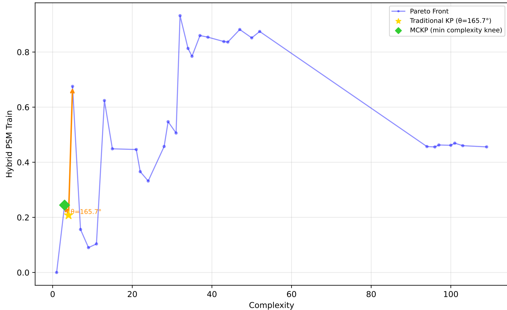
1096_FacultySalaries - Run 10 - SVP - Hybrid PSM Train \lambda_1=1.00, \lambda_2=0.00, \lambda_3=0.00 | Difficulty: 1.00 | Method: hmr
