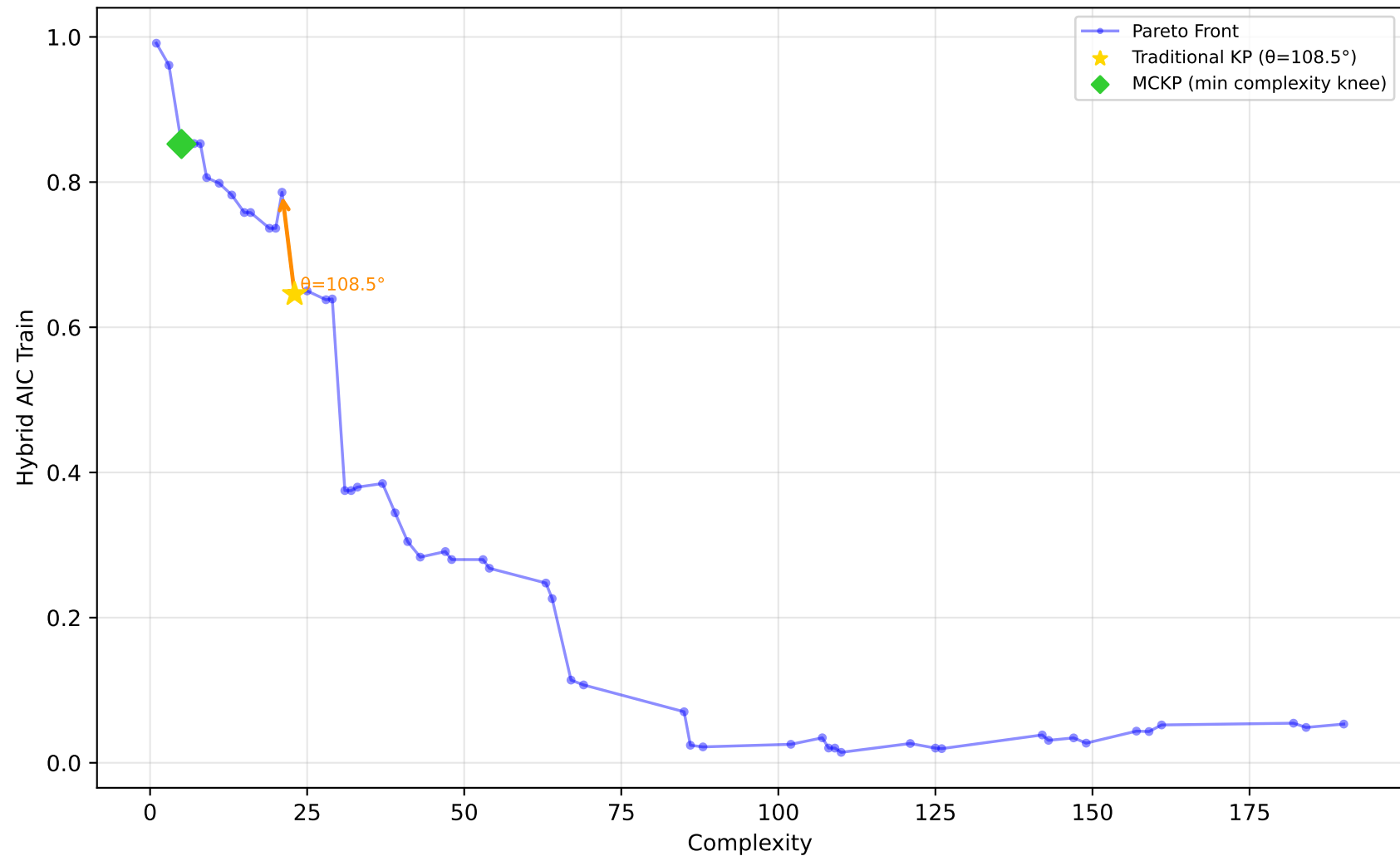
1096_FacultySalaries - Run 11 - MVP - Hybrid AIC Train \lambda_1=0.10, \lambda_2=0.00, \lambda_3=0.00 | Difficulty: 0.14 | Method: mckp
