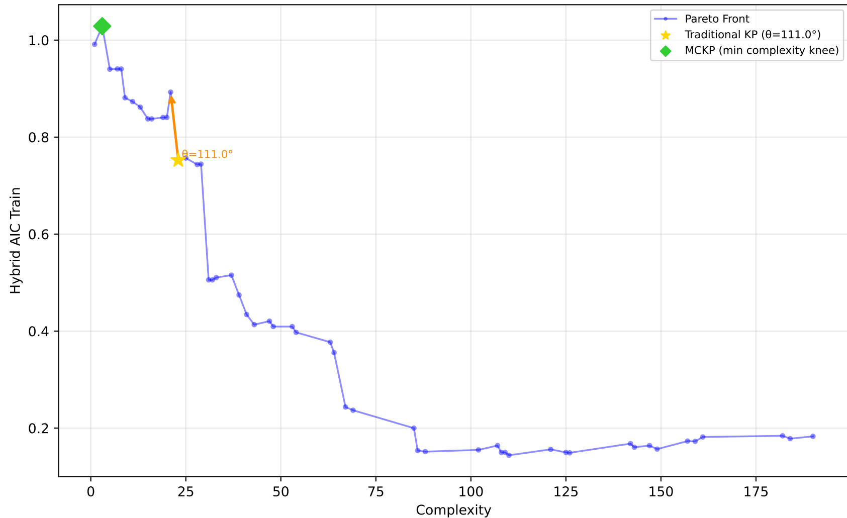
1096_FacultySalaries - Run 11 - MVP - Hybrid AIC Train \lambda_1=1.00, \lambda_2=0.00, \lambda_3=0.00 | Difficulty: 0.14 | Method: mckp
