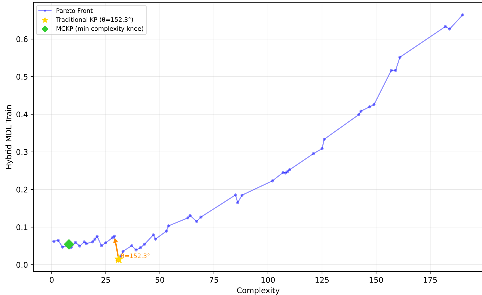
1096_FacultySalaries - Run 11 - MVP - Hybrid MDL Train \lambda_1=0.10, \lambda_2=0.00, \lambda_3=0.00 | Difficulty: 0.14 | Method: mckp
