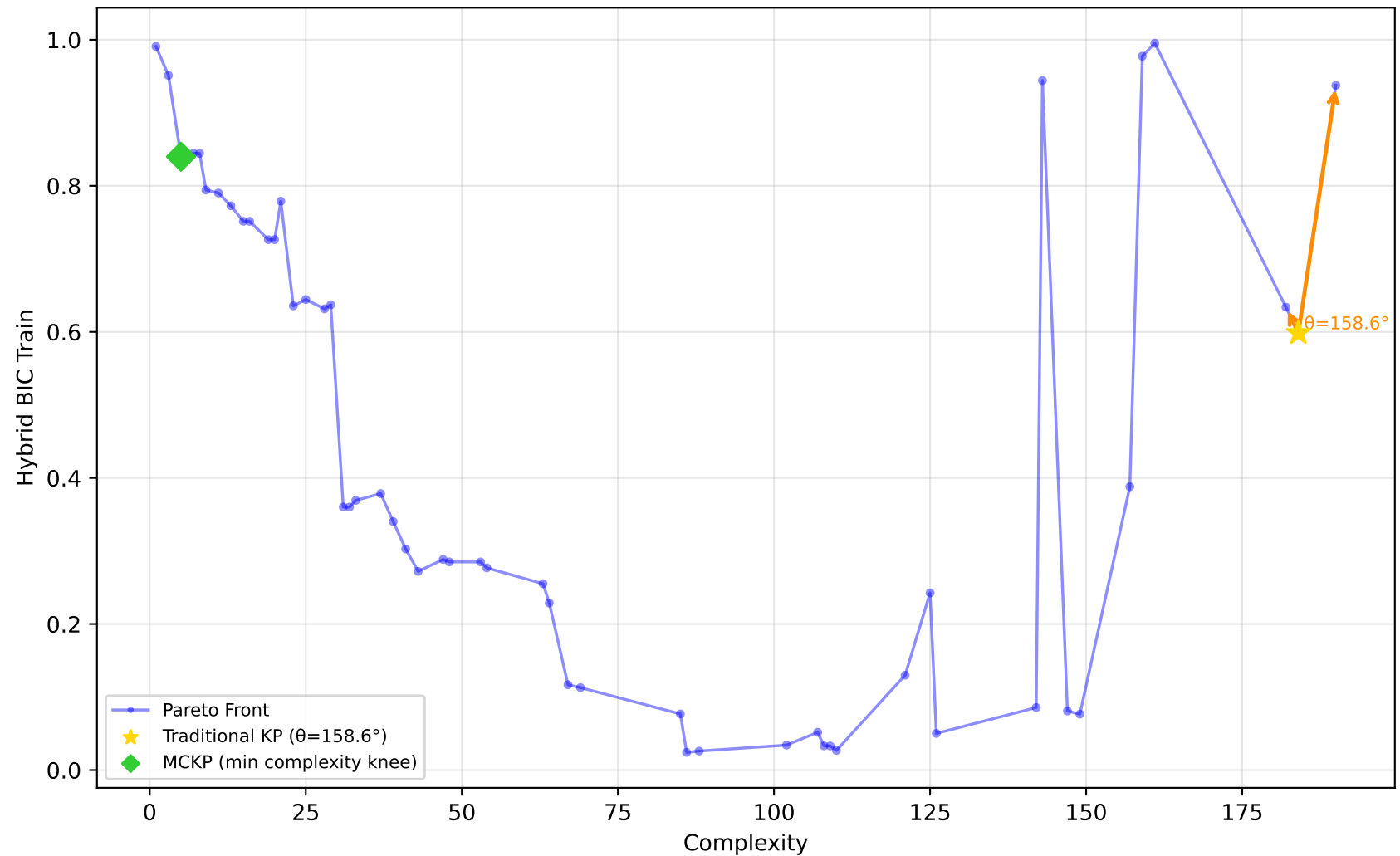
1096_FacultySalaries - Run 11 - SVP - Hybrid BIC Train \lambda_1=0.00, \lambda_2=0.90, \lambda_3=0.00 | Difficulty: 0.14 | Method: mckp
