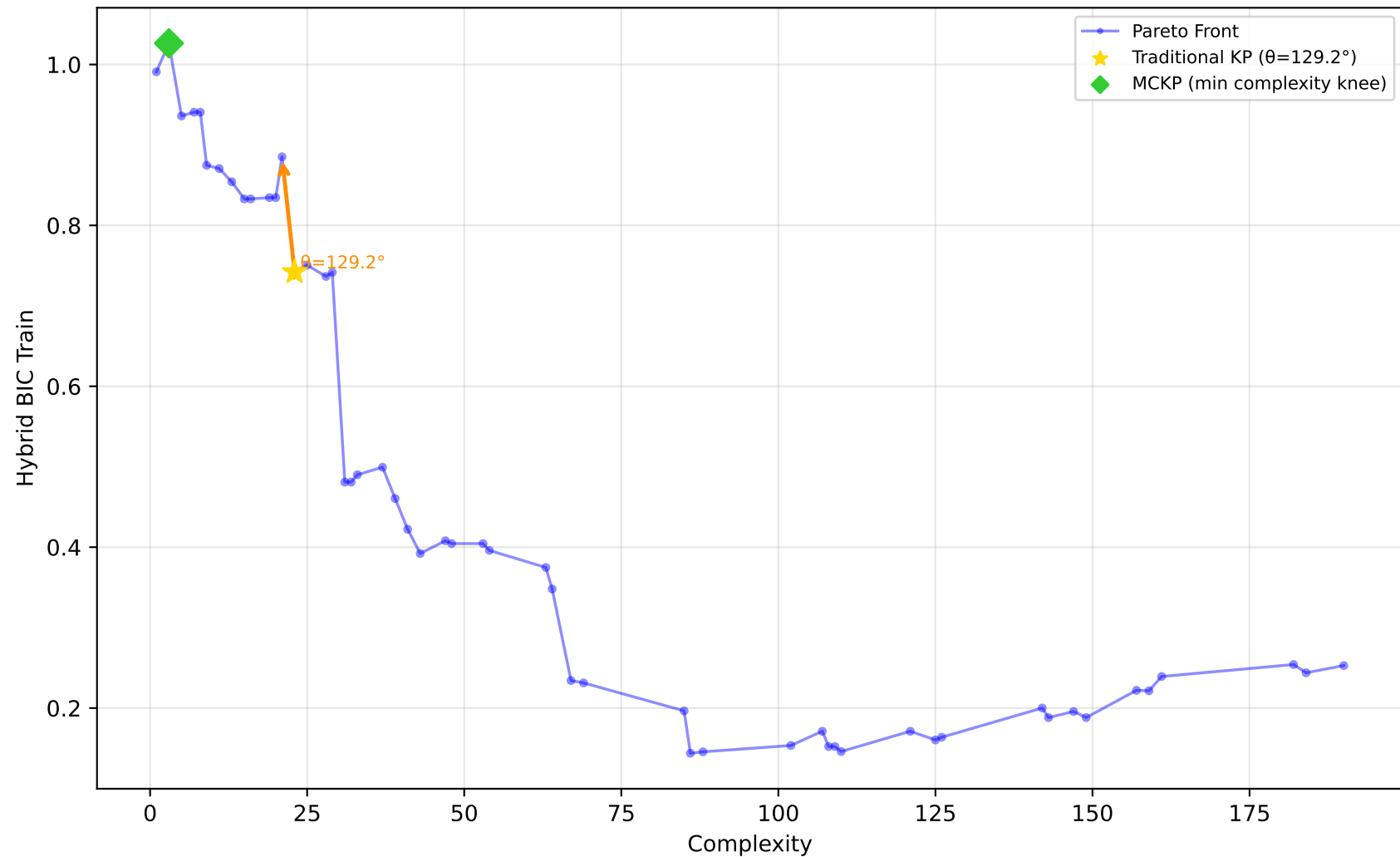
1096_FacultySalaries - Run 11 - SVP - Hybrid BIC Train \lambda_1=1.00, \lambda_2=0.00, \lambda_3=0.00 | Difficulty: 0.14 | Method: mckp
