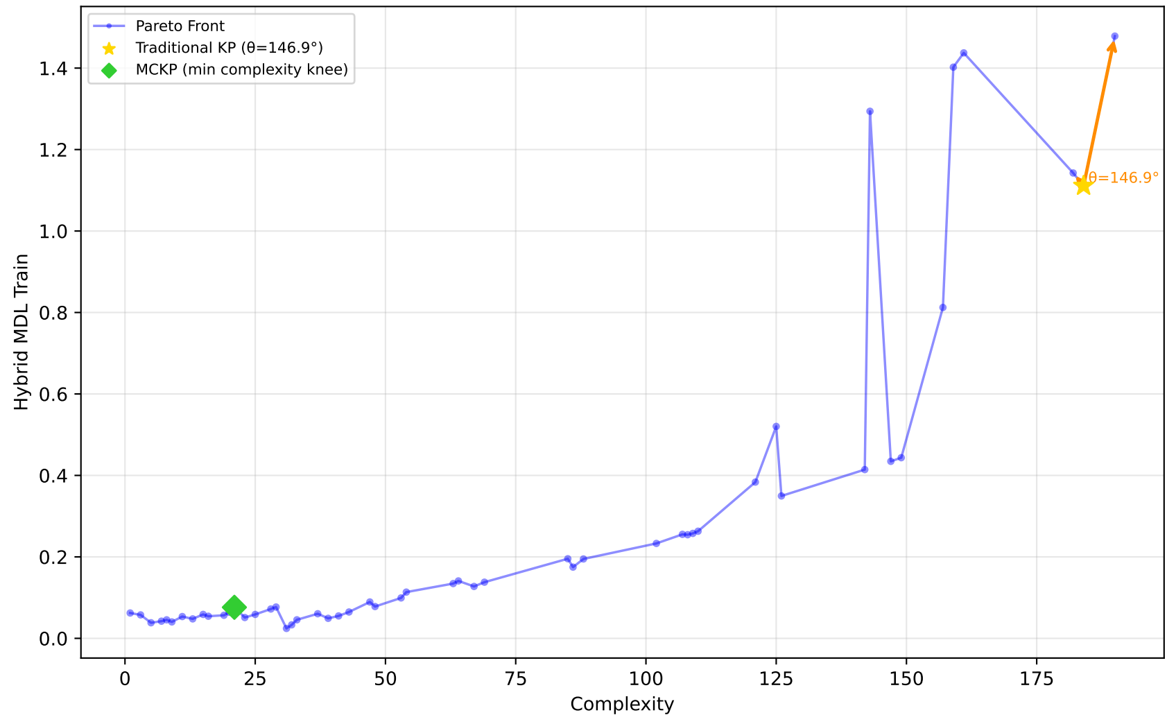
1096_FacultySalaries - Run 11 - SVP - Hybrid MDL Train \lambda_1=0.00, \lambda_2=0.90, \lambda_3=0.00 | Difficulty: 0.14 | Method: mckp
