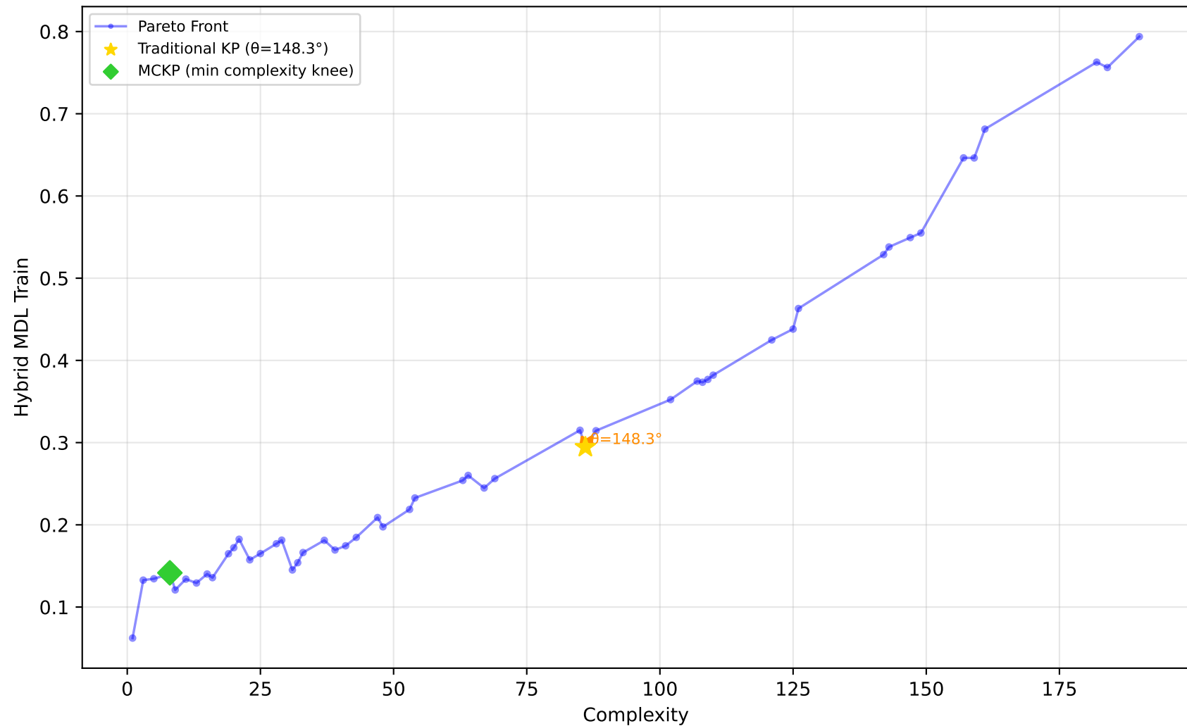
1096_FacultySalaries - Run 11 - SVP - Hybrid MDL Train \lambda_1=1.00, \lambda_2=0.00, \lambda_3=0.00 | Difficulty: 0.14 | Method: mckp
