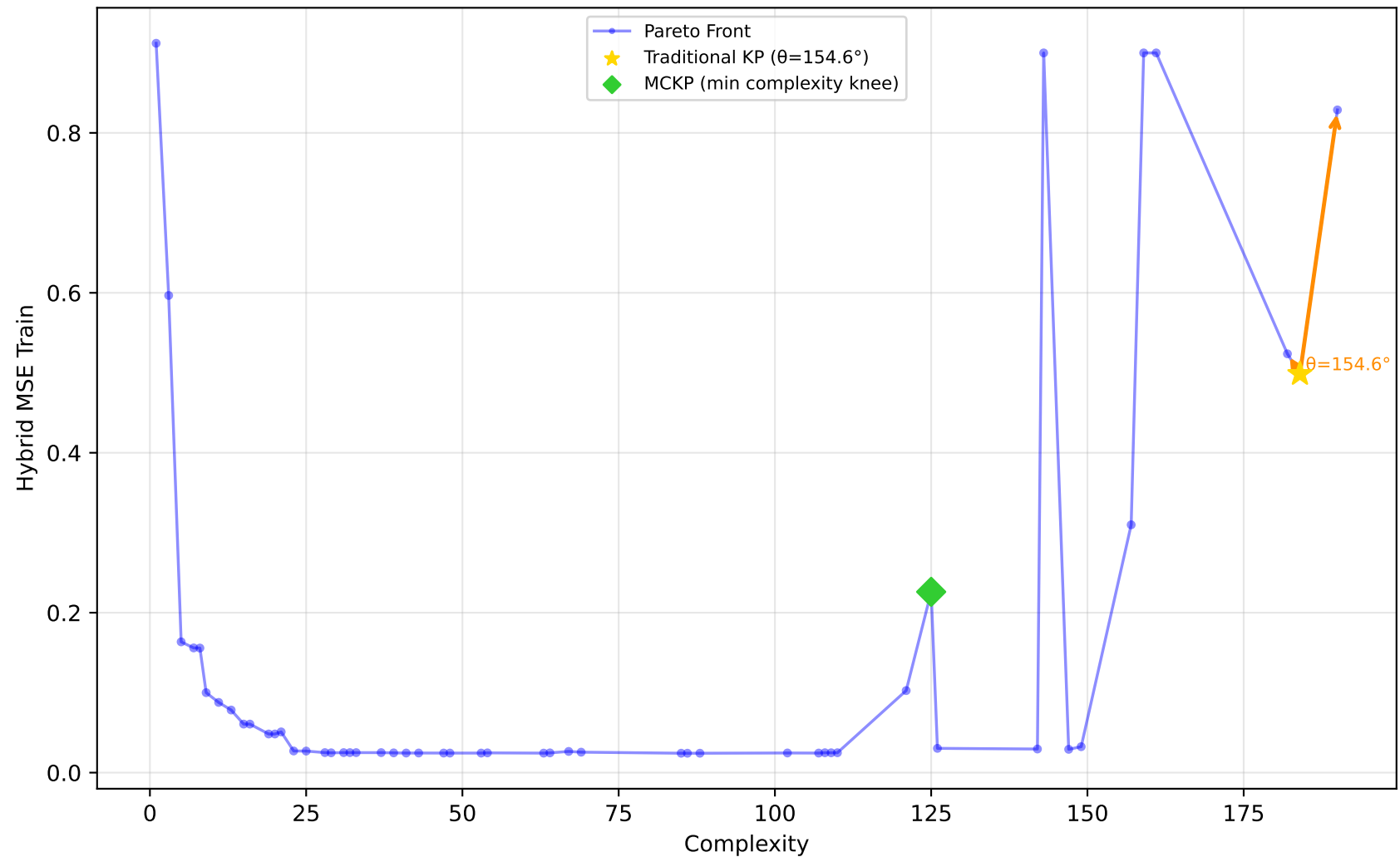
1096_FacultySalaries - Run 11 - SVP - Hybrid MSE Train \lambda_1=0.00, \lambda_2=0.90, \lambda_3=0.00 | Difficulty: 0.14 | Method: mckp
