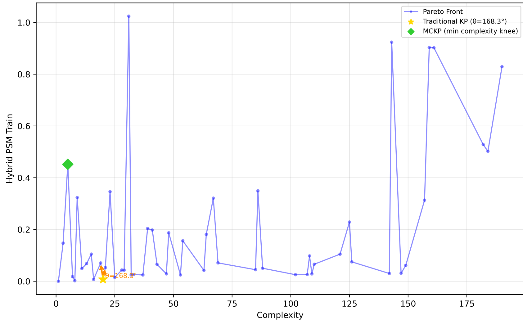
1096_FacultySalaries - Run 11 - SVP - Hybrid PSM Train \lambda_1=0.00, \lambda_2=0.90, \lambda_3=0.00 | Difficulty: 0.14 | Method: mckp
