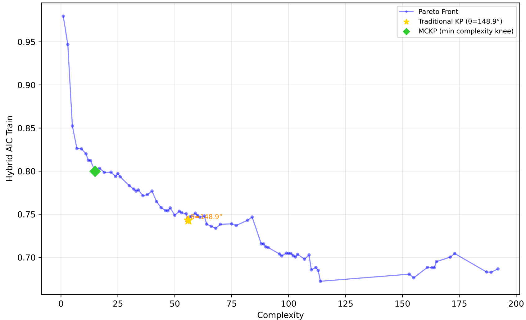
1096_FacultySalaries - Run 12 - MVP - Hybrid AIC Train \lambda_1=0.10 , \lambda_2=0.00 , \lambda_3=0.00 | Difficulty: 1.00 | Method: hmr
