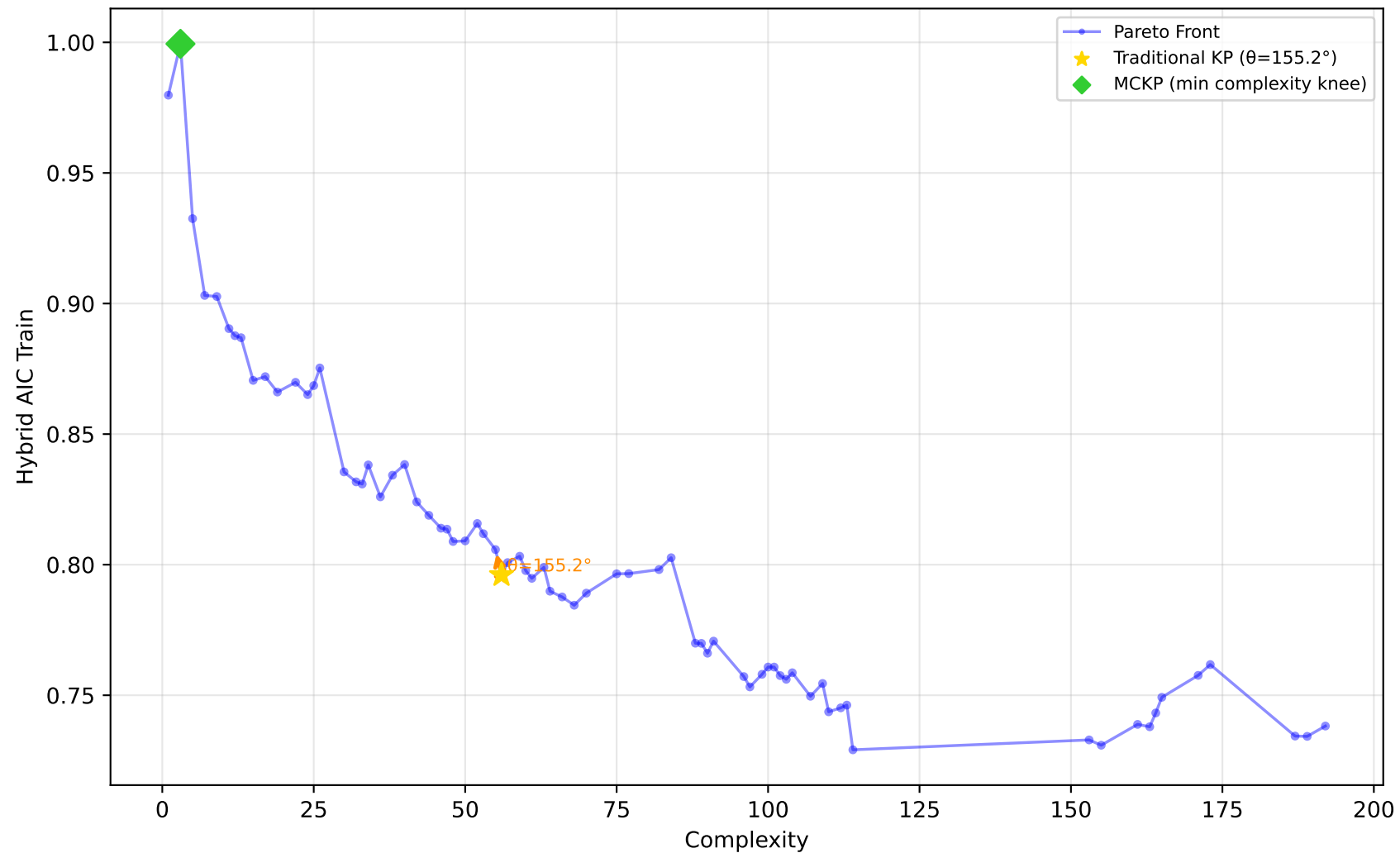
1096_FacultySalaries - Run 12 - MVP - Hybrid AIC Train \lambda_1=1.00 , \lambda_2=0.00 , \lambda_3=0.00 | Difficulty: 1.00 | Method: hmr
