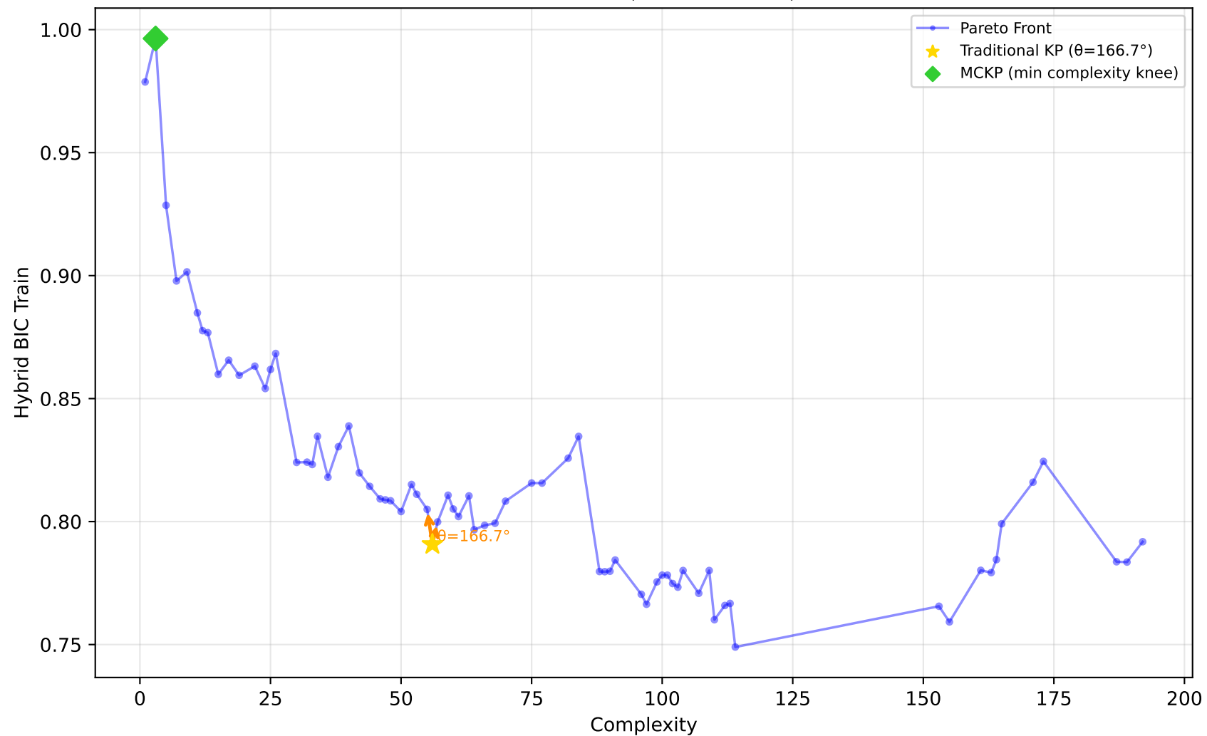
1096_FacultySalaries - Run 12 - MVP - Hybrid BIC Train \lambda_1=1.00 , \lambda_2=0.00 , \lambda_3=0.00 | Difficulty: 1.00 | Method: hmr
