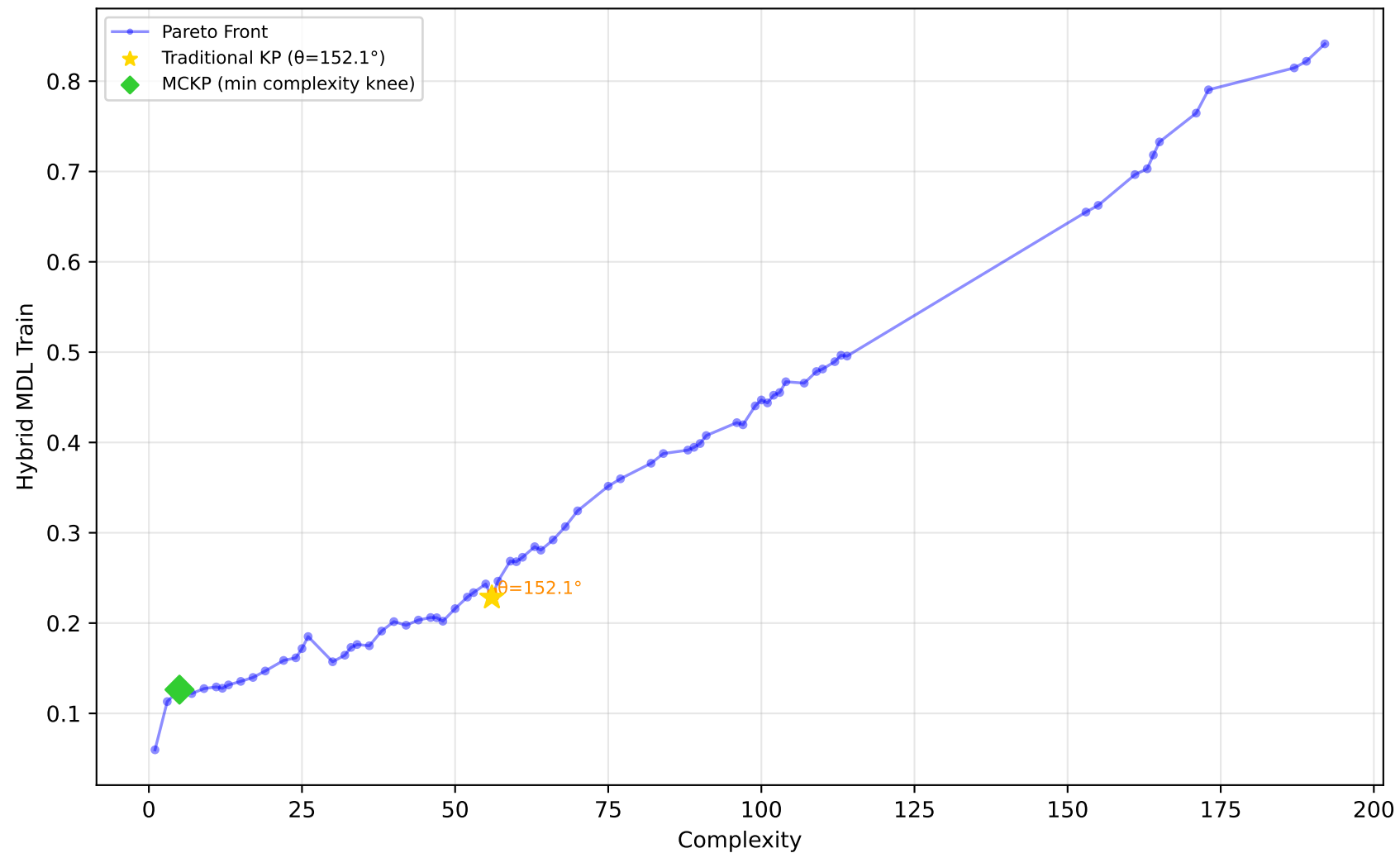
1096_FacultySalaries - Run 12 - MVP - Hybrid MDL Train \lambda_1=1.00, \lambda_2=0.00, \lambda_3=0.00 | Difficulty: 1.00 | Method: hmr
