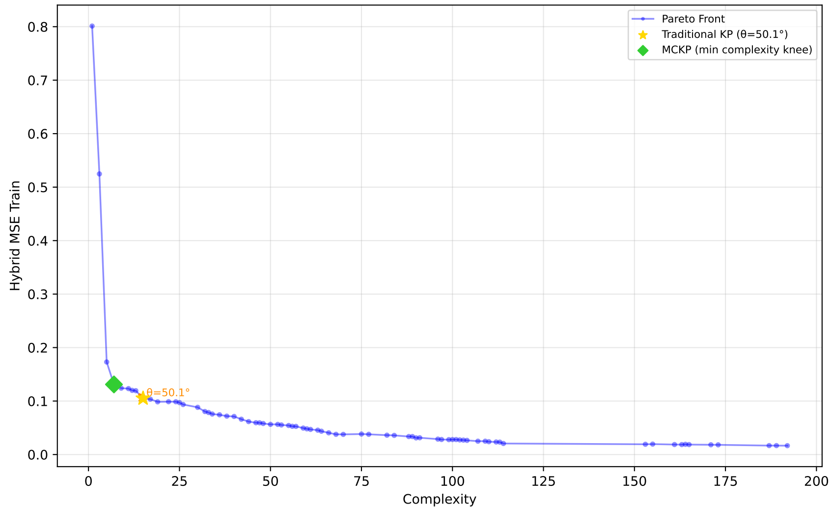
1096_FacultySalaries - Run 12 - MVP - Hybrid MSE Train \lambda_1=0.10, \lambda_2=0.00, \lambda_3=0.00 | Difficulty: 1.00 | Method: hmr
