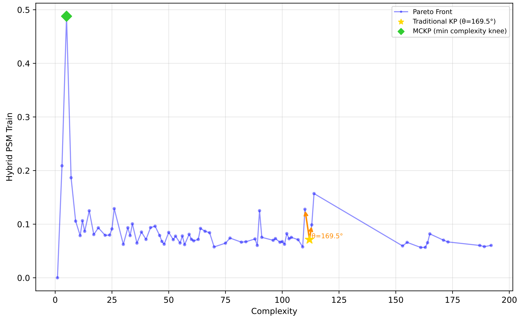
1096_FacultySalaries - Run 12 - MVP - Hybrid PSM Train \lambda_1=1.00 , \lambda_2=0.00 , \lambda_3=0.00 | Difficulty: 1.00 | Method: hmr
