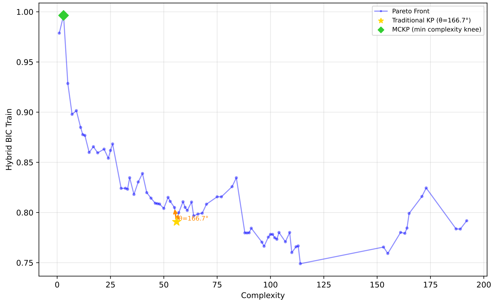
1096_FacultySalaries - Run 12 - SVP - Hybrid BIC Train \lambda_1=1.00 , \lambda_2=0.00 , \lambda_3=0.00 | Difficulty: 1.00 | Method: hmr
